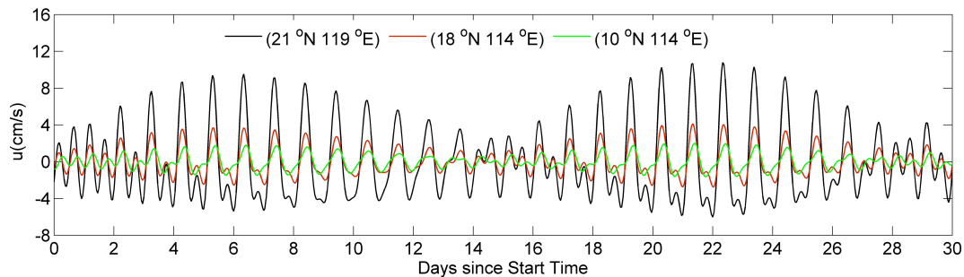
Fig. 1. Fig. A1. Time series of the barotropic tidal velocity predicted from TPXO 7.1 for three locations: (21°N, 119°E), (18°N, 114°E), and (10°N, 114°E).
