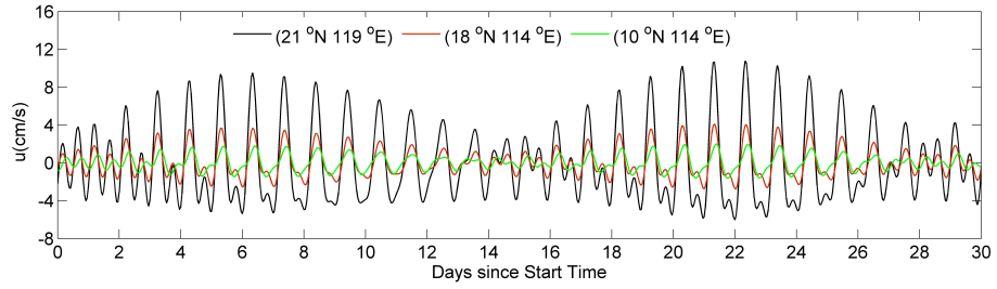
Fig. 1. Fig. A1. Time series of the barotropic tidal velocity predicted from TPXO 7.1 for three locations: (21oN, 119oE), (18oN, 114oE), and (10oN, 114oE).
