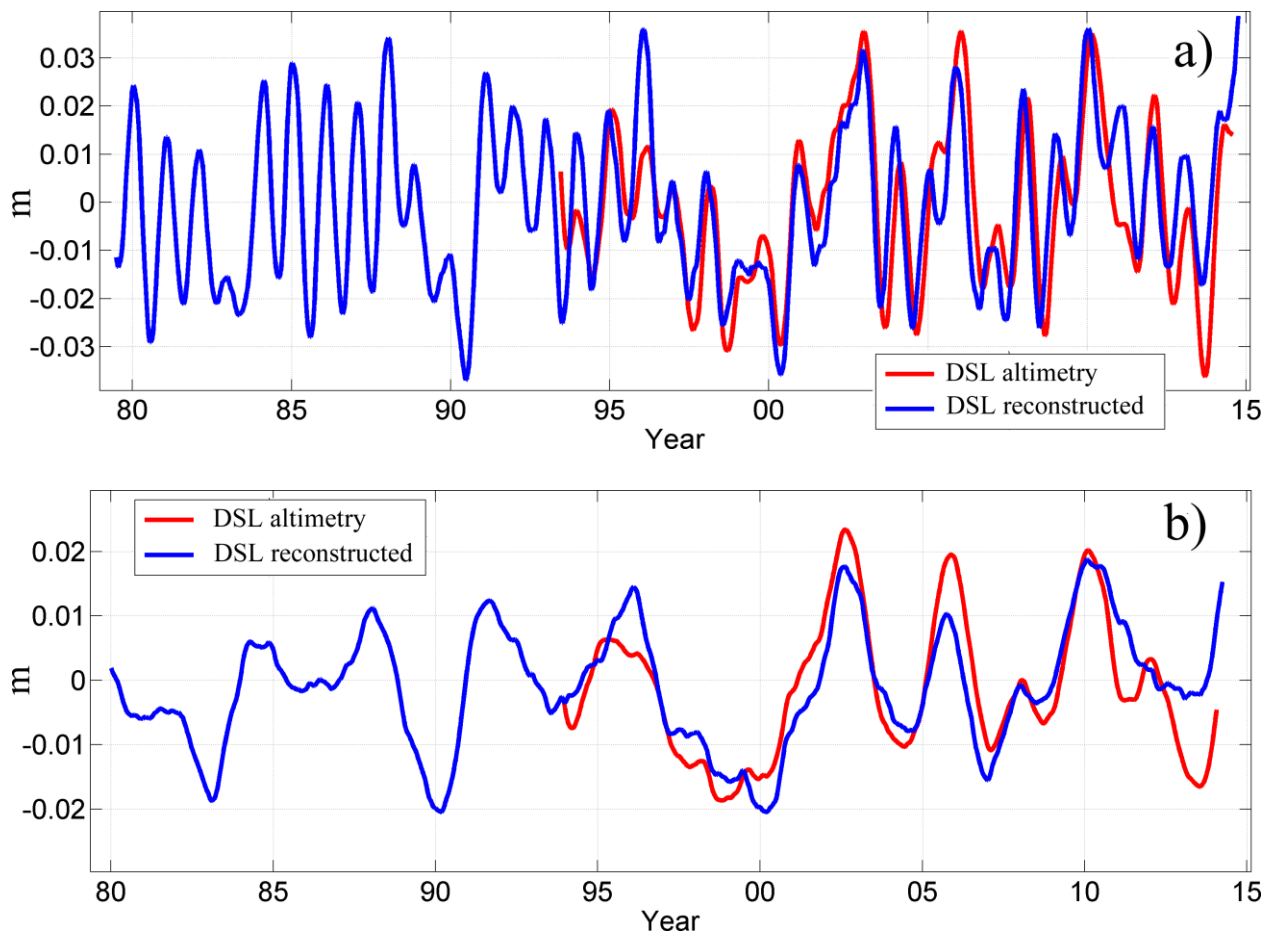
10 Figure 10: The time series of the altimetry-derived DSL (red curve) and DSL at 33.2^{\circ}E, 44.7^{\circ}N reconstructed from the wind curl (blue curve): the time series are smoothed (a) with a 90-day moving average and (b) with a 365-day moving average.
