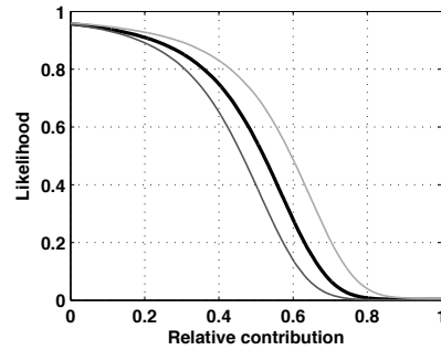
Figure 2. Likelihood—Thick black curve is the likelihood that the barystatic contribution to ENSO-related GMSL changes exceeds a certain fraction of the sum of barystatic and steric terms based on Monte Carlo runs, where the steric term is evaluated based on the average of the SIO and IPRC gridded data products. The thin dark gray (light gray) curve is that same likelihood but with the steric term assessed using only the SIO (IPRC) product.
