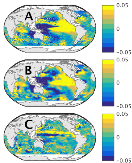
Figure 5. (a) Spatial pattern of nonseasonal anomalous Argo steric sea level (relative to 2005–2015 with linear trends and annual cycles removed) computed from the SIO gridded dataset over the last six months (July–December) of 2015. (b) As in (a) but computed from the IPRC gridded dataset. (c) Spatial pattern of the difference between the two gridded datasets (i.e., SIO minus IPRC). All panels have units of cm steric sea level.
