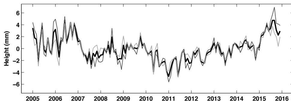
185 Figure R1: Time series of nonseasonal anomalous thermosteric sea level from: average of 186 SIO and IPRC products (black); SIO product (dark gray); and IPRC data (light gray).
