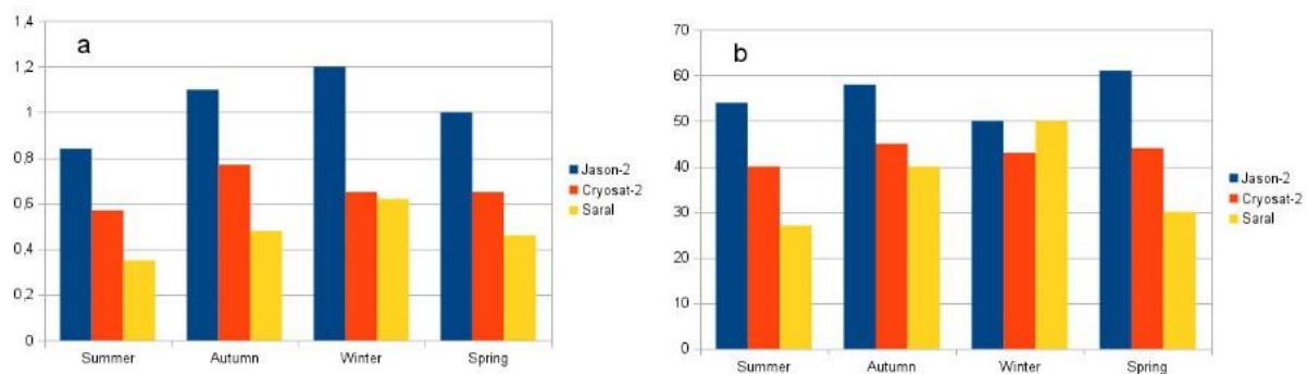
Figure 4. a) Seasonal noise levels (in 10^{-3} \text{ m}^2/\text{cpkm} ) for Jason-2 (blue), Cryosat-2 SAR mode (orange) and Saral/AltiKa (yellow) derived from along-track wavenumber spectra. b) Seasonal observational limits in terms of wavelength (in km) where the signal-to-noise is > 1 for each altimeter mission. Table 1 gives the number of sections used.
