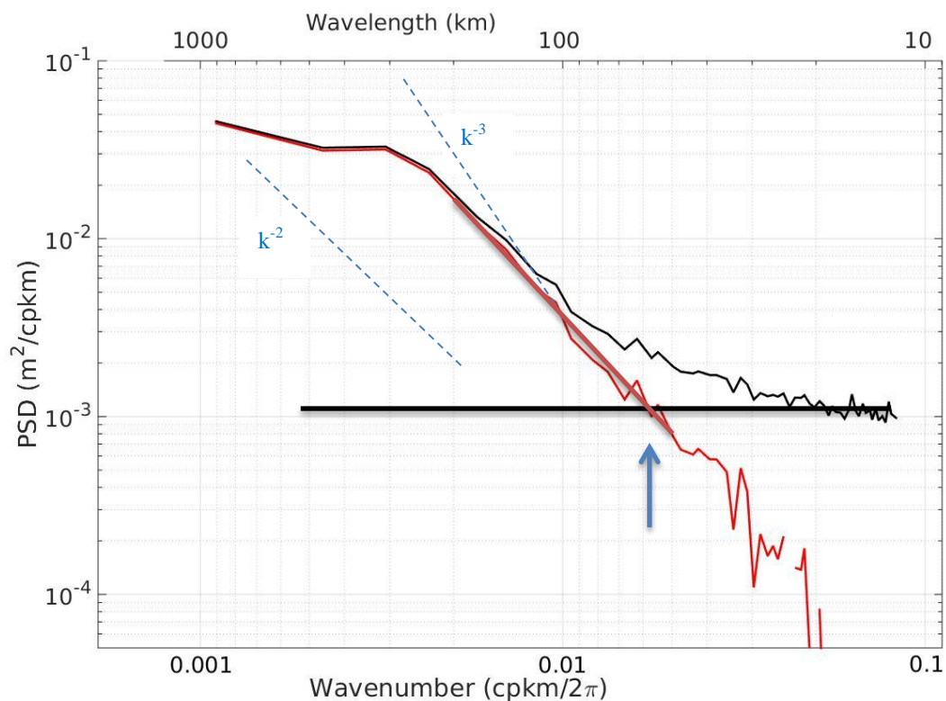
Figure 2. Mean wavenumber spectra (power spectral density) for Jason-2 sea level anomalies, averaged over all tracks in the NW Mediterranean Sea > 50 km from the coast (black line) for the period 1 Apr 2013 – 30 Apr 2014. The estimated noise level is shown as the thick black line. The unbiased spectra (thin red line) is obtained by subtracting this constant noise from the original spectra. The spectral slope (thick red line) is calculated between 50 and 200 km wavelength. The intersection between these two curves represents the mesoscale observational limit (blue arrow), above which the mean signal-to-noise ratio is >1.
