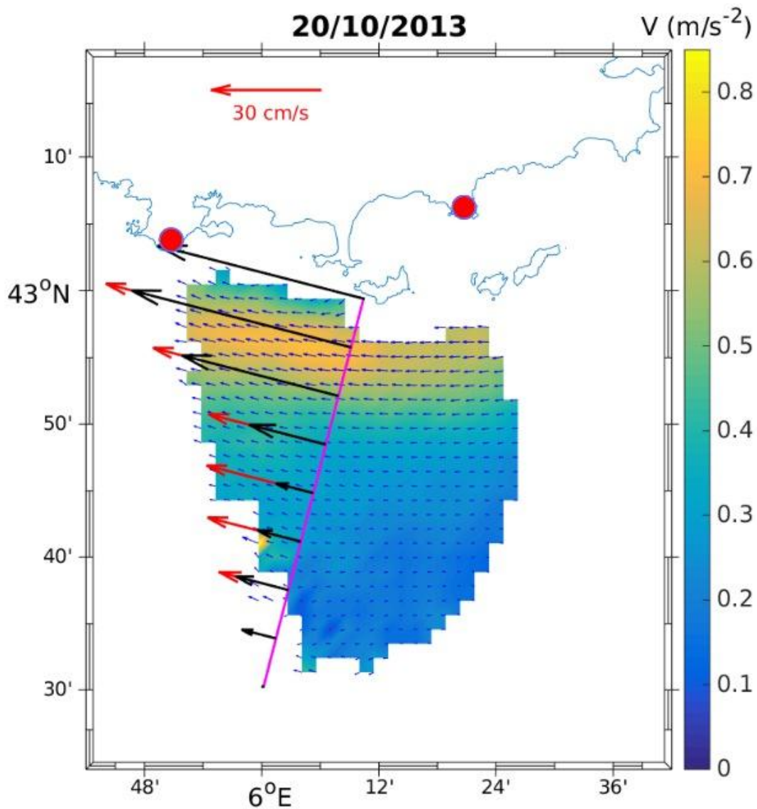
Figure 10. HF radar surface currents near Toulon for one date (20 Oct 2013); direction with small blue arrows, current speed is in colour. Saral track #302 is marked in pink. 1 Hz cross-track geostrophic currents from Saral altimetry are in black, the HF radar total currents projected in the altimetric cross-track direction are in red. The current scale of 30 cm/s is associated with the projected currents.
