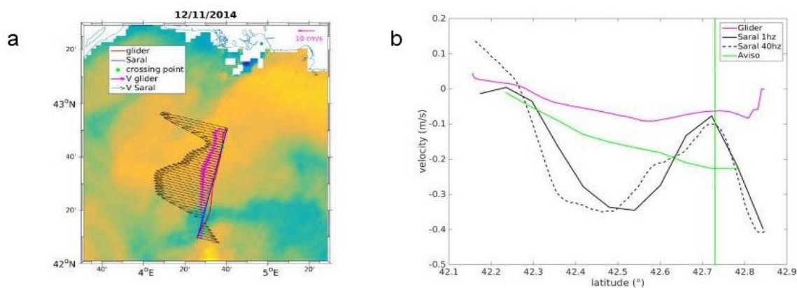
Figure 7. a) Collocated Saral track 388 and currents (in black) and glider track and currents (in pink), overlaid with a satellite SST plot on 12 Nov 2014. b) along-track comparison of geostrophic velocities for the glider (including the drift velocities) in pink, and filtered Saral data in black. Mapped AVISO altimeter data, interpolated back onto the altimeter track, are in green. Green vertical line shows the position when the altimeter data and gliders are collocated. Daily SST fields at 0.02° resolution from CLS.
