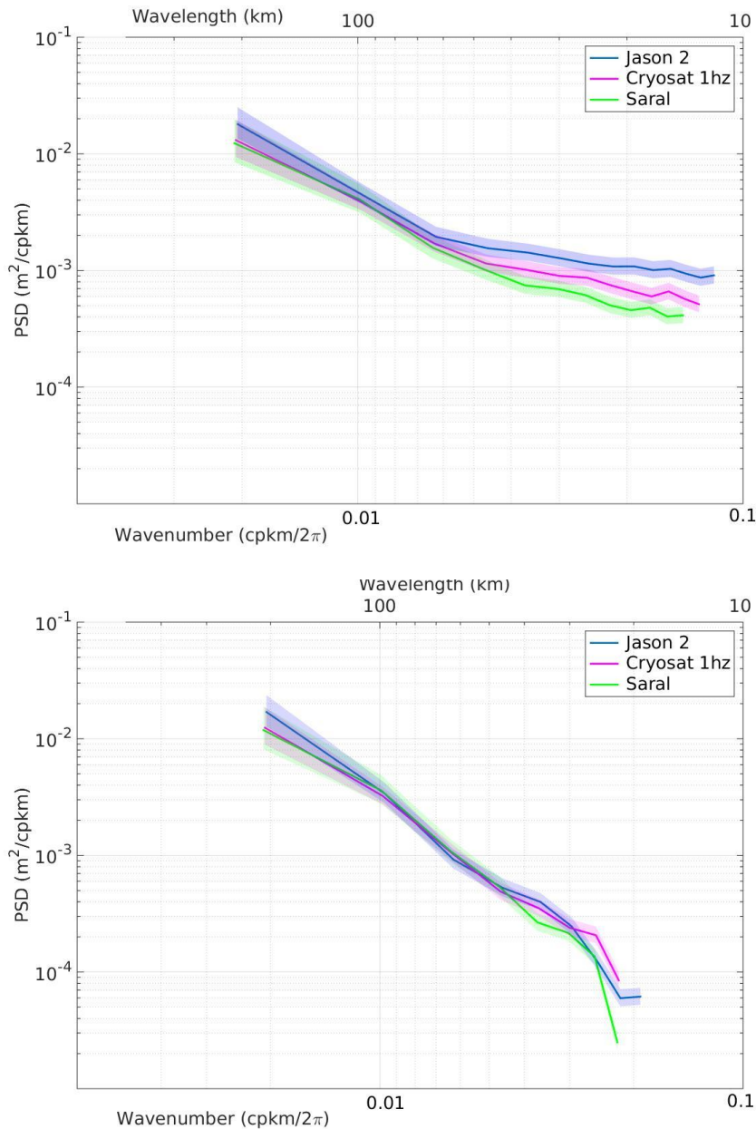
Figure 3 a) Mean wavenumber spectra (power spectral density) for the three altimeter missions, averaged over all tracks in the NW Mediterranean Sea > 50 km from the coast for the period 1 Apr 2013 – 30 Apr 2014. Jason-2 is in blue, Saral in green, Cryosat-2 SAR 1 hz data in pink. b) The unbiased spectra with a constant noise level removed, with a mean k^{-2.5} spectral slope. Shading represents the error bars, based on a \chi^2 test with the number of degrees of freedom being wavenumber dependant. Table 1 gives the number of sections used.
