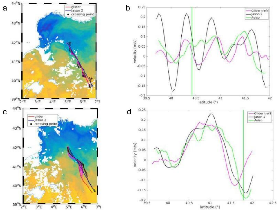
Figure 6. a) Collocated Jason-2 track and currents (in black) and glider track and currents (in pink) for the southbound leg, overlaid with a satellite SST plot on 1 Oct 2012. b) along-track comparison of geostrophic velocities for the glider (including the drift velocities) in pink, and filtered alongtrack Jason-2 data in black. Mapped AVISO altimeter data, interpolated back onto the Jason-2 track, are in green. Green vertical line shows the position when the Jason-2 data and gliders are collocated in time. c) and d), same but for the northbound section with SST fields from the 21 Oct 2012. 48h SST fields at 0.02° resolution from CLS.
