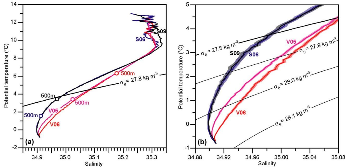
Figure 5. \theta -S diagrams for four standard stations based on 73 occupations at stations V05 (magenta) and V06 (red) simultaneously and on 54 occupations at stations S06 (blue) and S09 (black) simultaneously in the period 1996 – 2010. (a) Average \theta -S traces for the whole water column with conditions at 500 m depth indicated by circles. (b) Expanded view of waters colder than 5 °C with the average for each station shown as a coloured line surrounded by a shaded area in the same colour representing the average \pm 1 standard error. Station locations are shown on Fig. 1 and Fig. 2a.
