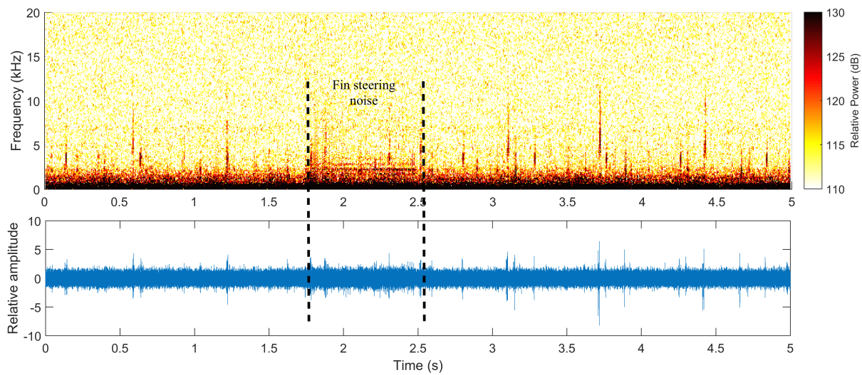
Figure 9. Spectrogram (top) and time series (bottom) of 5 seconds of data showing an example of noise (between dashed lines) produced by fin steering in the glider, with sperm whale echolocation clicks (narrow vertical bars) around it.
