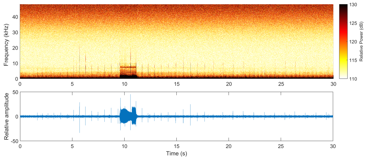
Figure 11. Spectrogram (top) and time series (bottom) showing an example of noise produced by the pitch pump, which makes small adjustments to the battery position during a dive. Sperm whale echolocation clicks can also be observed in this sequence, especially in the time series data.
