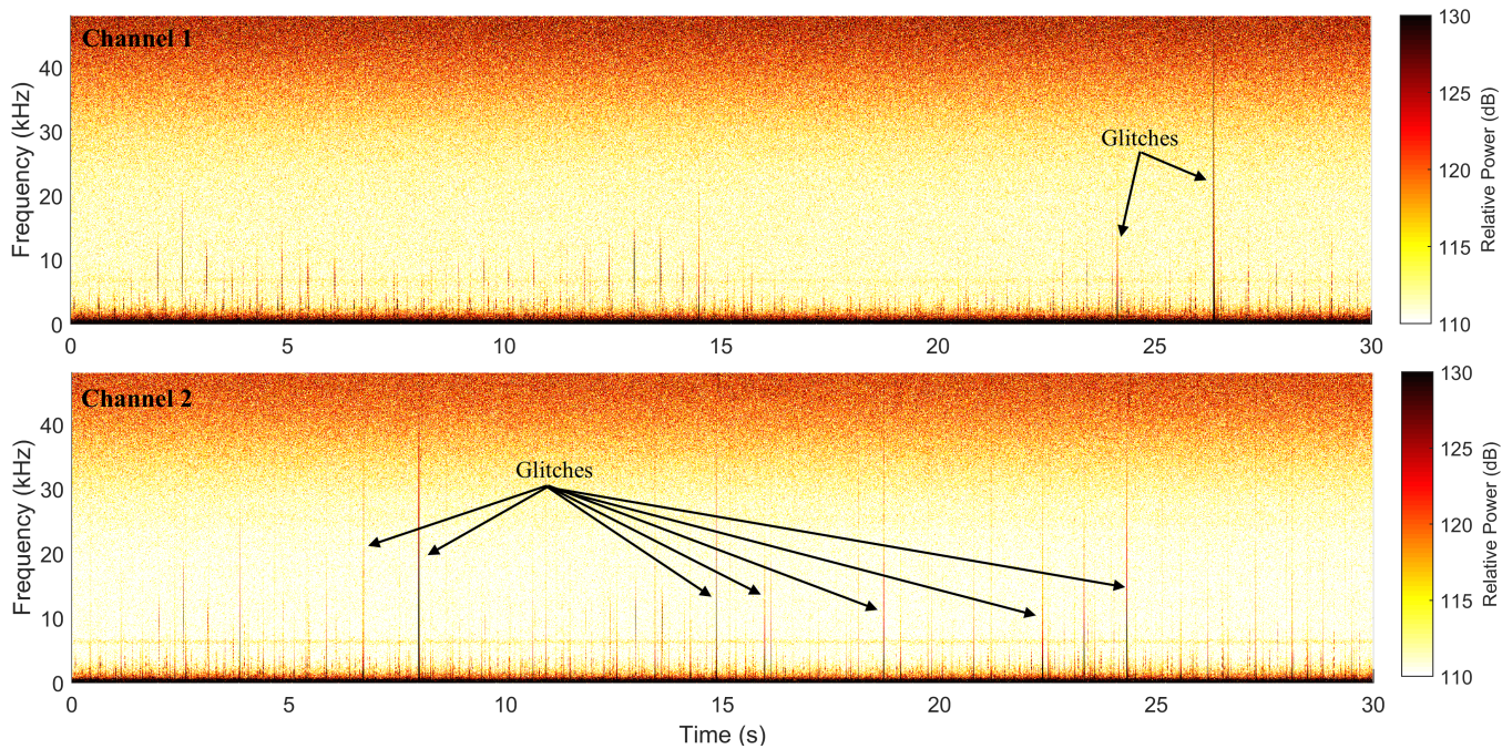
Figure 7. Spectrogram of 30 seconds of data recorded on channel 1 (top) and channel 2 (bottom) showing the occurrence of glitches for the same period. While there were only two instances when glitches occurred on channel 1, they showed up many times on channel 2 (only a few are actually shown).
