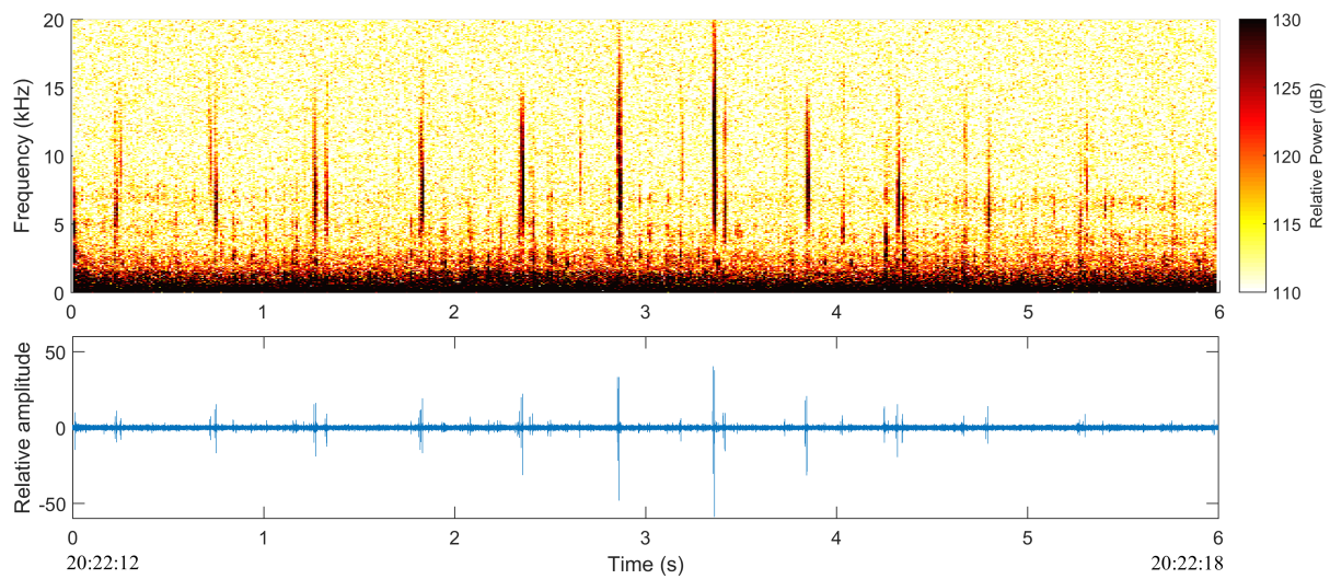
Figure 5. Example of possible sperm whale multipath arrivals - here evidenced by fainter clicks following the stronger first arrivals, more noticeable between 2-5 s and shown on both spectrogram (top) and waveform (bottom) of 6 seconds of data from channel 1.
