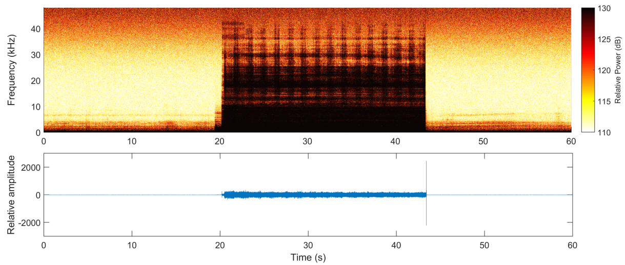
Figure 10. Spectrogram (top) and time series (bottom) showing an example of the noise produced by battery movement and volume piston. The volume piston noise starts just before 20 s, and is then masked by the battery movement noise.
