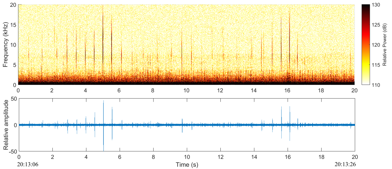
Figure 3. Spectrogram (top) and waveform (bottom) of 20 seconds of data recorded on channel 1 of file 06 showing sperm whale regular clicks (narrow vertical bars). Time stamps are local time (CEST) on 09 June 2014. The relative amplitude corresponds to the amplitude in dB minus the hydrophone sensitivity of -161.4 dB re 1 \mu\text{Pa}/\text{V} .
