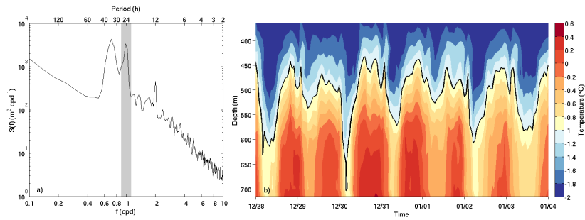
Figure 13. a) Power spectral density of the height above the bottom of the -1^{\circ}\text{C} isotherm which indicates the transition between WW and WDW at M3. The diurnal tidal frequency band is marked in grey. b) Hovmöller diagram of low-pass filtered temperature at mooring M3 from 28 December to 4 January. The -1^{\circ}\text{C} isotherm is shown by a black line.
