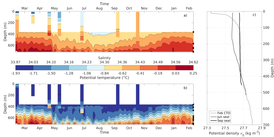
Figure 7. Hovmöller diagrams for a) salinity and b) temperature. The continuous records below approximately 350 m depth are the hydrographic time series of moored instruments at M3, acquired in 2009 (see Table 1). The mooring data have been low-pass filtered by applying a fourth order Butterworth filter removing variability at shorter periods than the cut-off period of 168 h (one week). Black triangles mark the depths of individual measurements. CTD profiles from ship (from the deployment cruise of mooring M3 in 2009, first profile) and seals (obtained in 2011 from within approximately 10 km distance to mooring M3, see Fig. 1) complement the mooring records. The width of the profiles is arbitrarily set to one week for clarity. Panel c) shows the seasonal development of potential density based on three of the temperature and salinity profiles near mooring M3.
