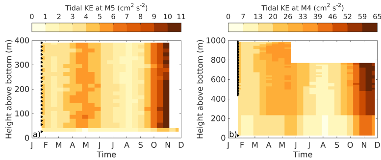
Figure 4. Diurnal tidal KE over time and depth at a) mooring M5 and b) mooring M4 on the continental slope, located above the 1900 m and 1050 m isobath, respectively . Black triangles mark the depths of individual measurements. Note the different scale for diurnal tidal KE and vertical axis in a) and b).
