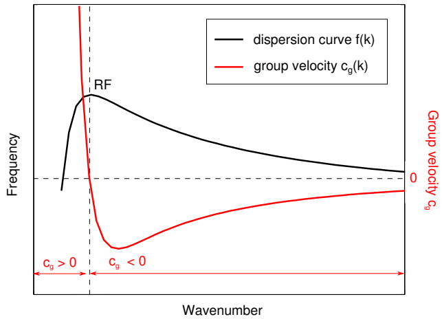
Figure 2. Illustration of a typical mode 1 CTW dispersion curve (black line) with the corresponding group velocity (red line). For small wavenumbers, the group velocity is positive, while it becomes negative for larger wavenumbers, i.e. indicating a change of direction of energy propagation. At the maximum of the dispersion curve (the resonant frequency, or “RF”), the group velocity vanishes and energy is trapped.
