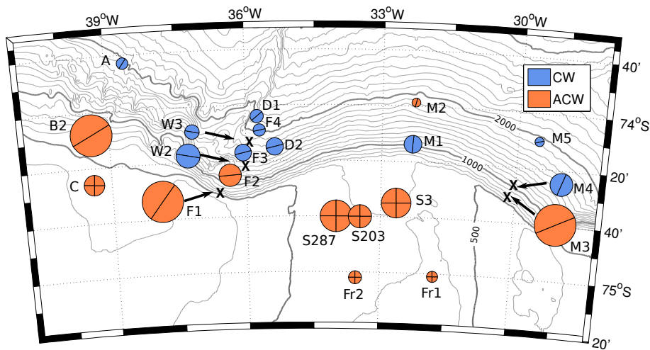
Figure 5. Map showing the maximum depth-averaged, diurnal tidal KE reached in austral summer . The area of the circles on the map is proportional to the square root of the maximum of depth-averaged, diurnal tidal KE reached in austral summer . Blue circles indicate a clockwise (CW) rotation of tidal currents at the K_1 frequency, red circles an anticlockwise (ACW) rotation, as inferred from harmonic analysis . The line through the circles indicates the orientation of the major axis (i.e. strongest tidal current). Tidal current ellipses with an aspect ratio (semi-minor/semi-major axis) of more than 0.8, i.e. close to circular, are marked with two crossing lines instead of a single line. At the location of mooring S2 with five years of measurements, the data for the deployment years 1987 (S287) and 2003 (S203) are presented. Some circles are displaced from their actual mooring locations (marked with “X”) for legibility.
