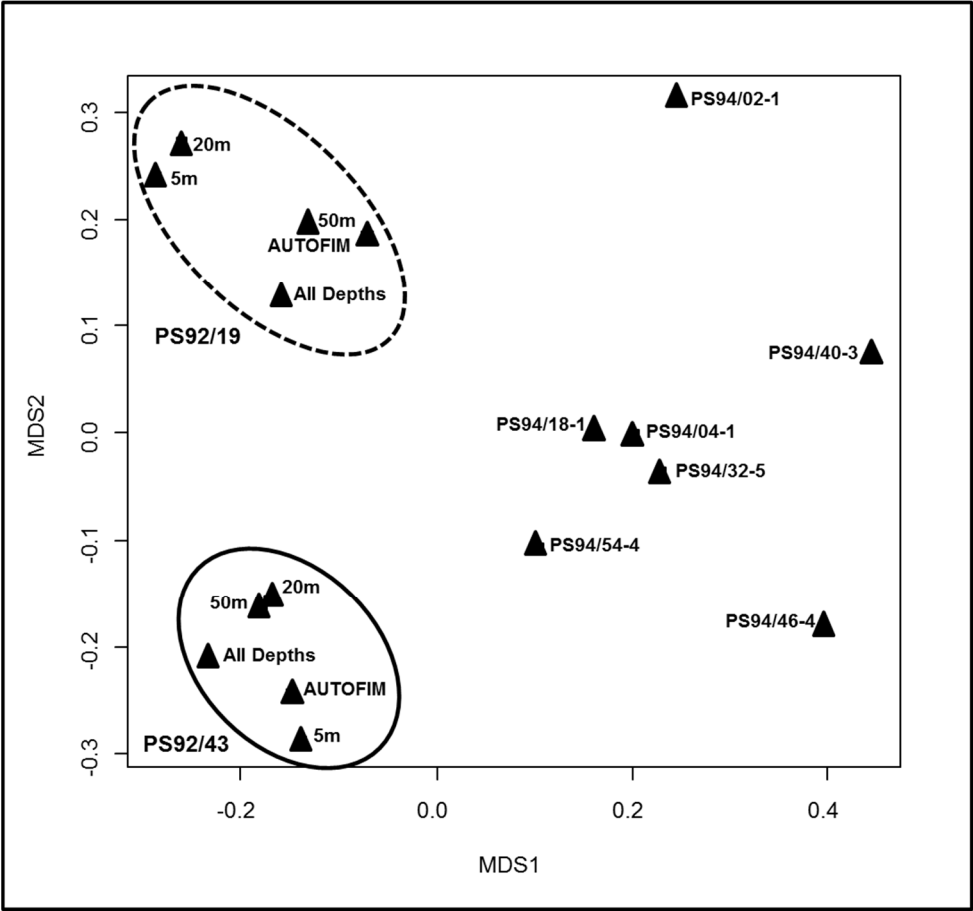
490 491 492 Fig. 3: MetaMDS Plot (non metric multidimensional scaling plot) of ARISA fingerprints generated from 493 samples collected via CTD and AUTOFIM. The closer the samples are located to each other in the metaMDS- 494 plot, the more similar are the ARISA-profiles of the samples. The label of the samples gives information on the 495 cruise leg (PSXX) and the station (/XX). Samples were collected during expeditions PS92 and PS 94 of RV 496 Polarstern to the Arctic Ocean during summer 2015. The samples collected during PS94 serve as an outgroup in 497 this analysis.
