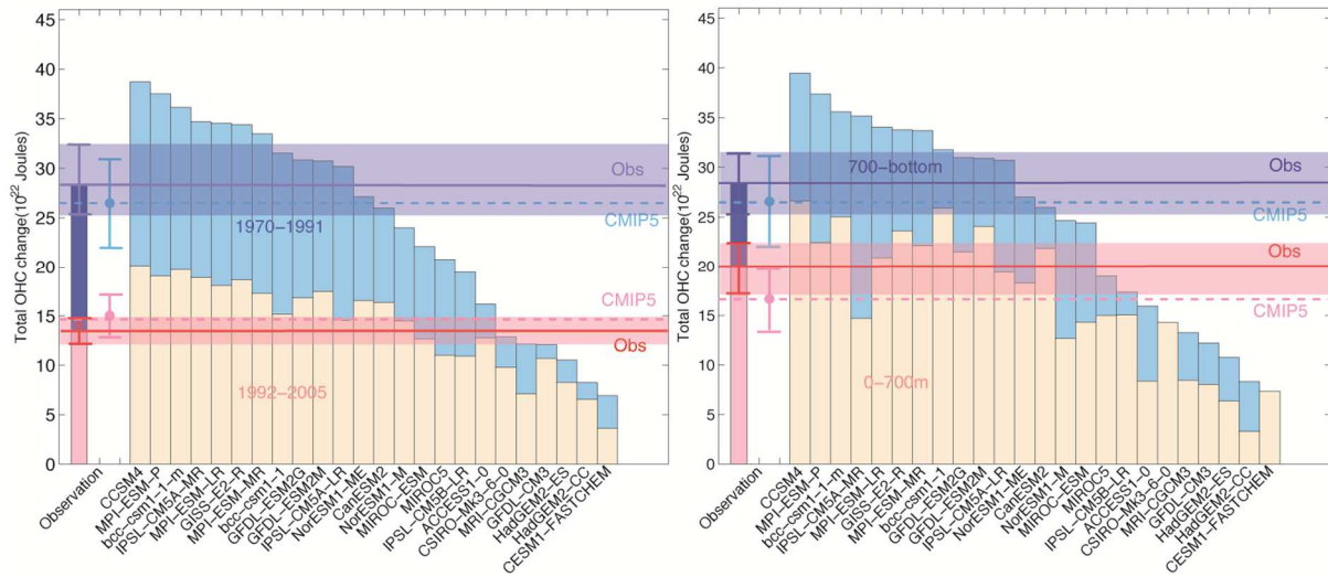
5 Figure 5. Comparison of full-depth OHC change between observation and CMIP5 models a). for two separate time periods: 1970-1991 (in blue bars) and 1992-2005 (in red bars) and b). for two vertical layers: 0-700m (in red bars) and 700m-bottom (in blue bars). The medians of the observational total OHC changes are shown in solid lines, compared with the model results in dashed lines. Their 5%-95% confidence intervals are presented in error bars. The 5%-95% confidence intervals for observations are also shaded in light red and light blue. A quadratic fit to the entire pre-industrial control run was used to correct the CMIP5 time series for model drift.
