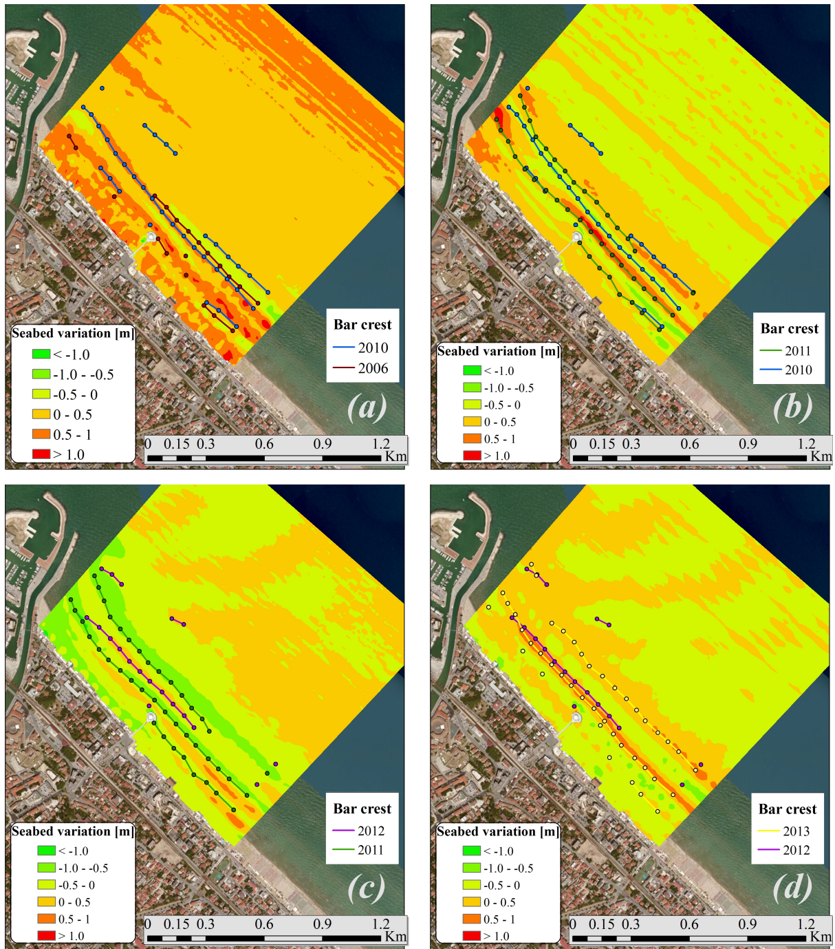
Figure 4. Sea bottom variation within time periods: (a) 2006–2010, (b) 2010–2011, (c) 2011–2012 and (d) 2012–2013. Colored lines show the bar-crest locations extracted from the cross-shore profiles.
