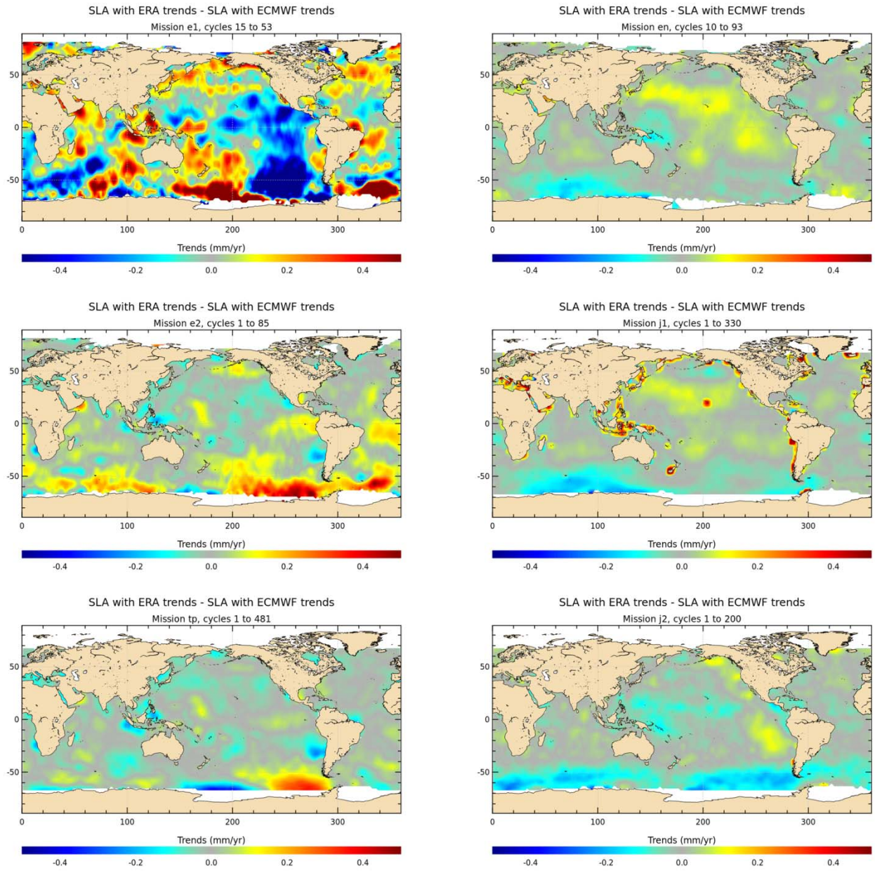
Figure 13: Maps of MSL trend differences using successively the DT correction derived from ERA-Interim and from ECMWF operational pressures fields (reference) for ERS-1, ERS-2 and TOPEX on left-hand panels, for Envisat, Jason-1 and Jason-2 on right-hand panel (mm/year).
