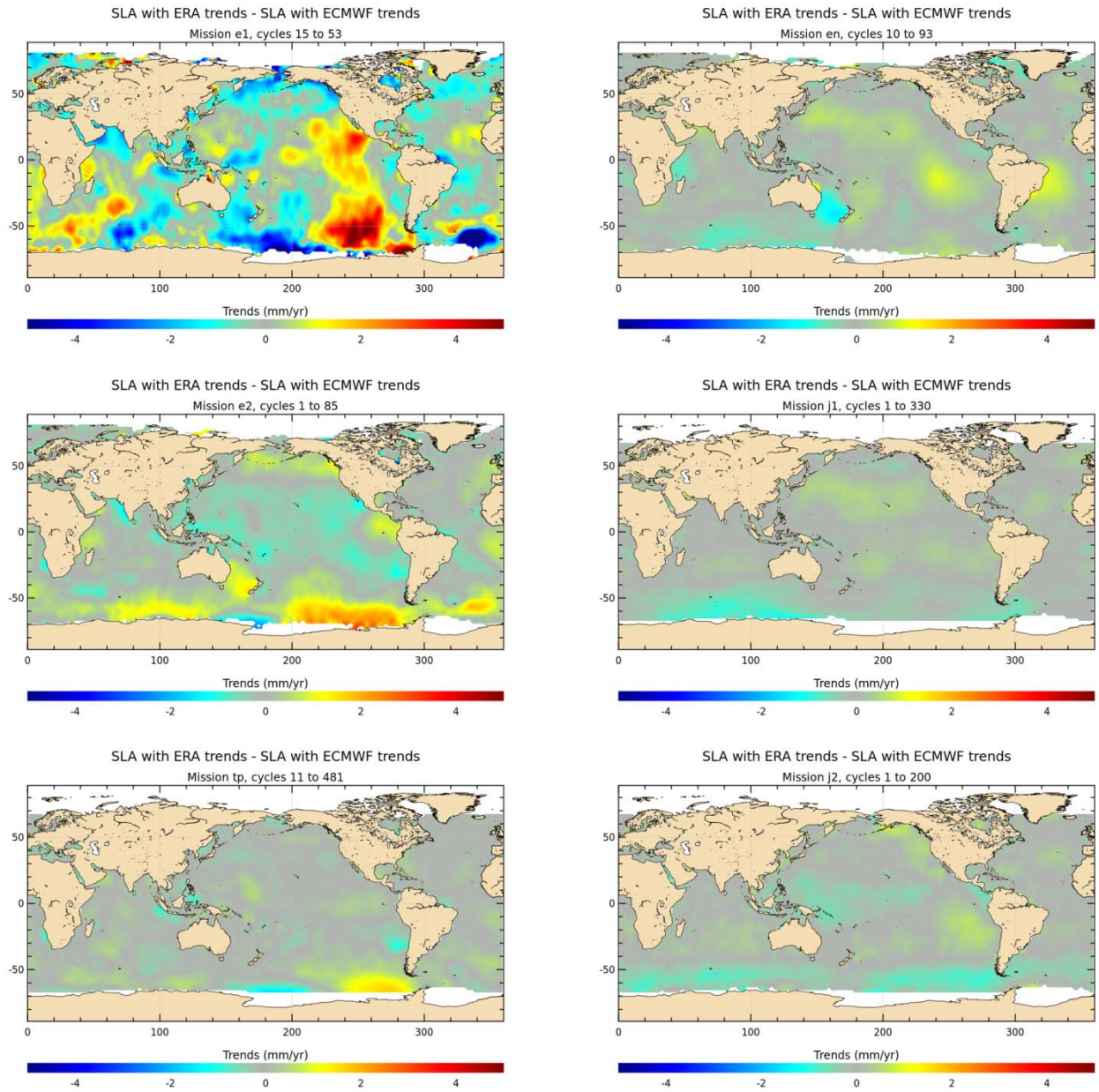
Figure 12: Maps of MSL trend differences using successively the DAC derived from ERA-Interim and from ECMWF operational pressures fields (reference) for ERS-1, ERS-2 and TOPEX on left-hand panels, for Envisat, Jason-1 and Jason-2 on right-hand panel (mm/year).
