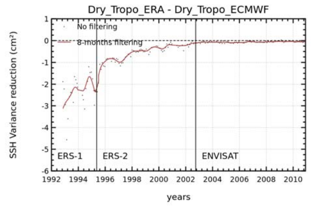
Figure 10: Temporal evolution of SSH variance differences at crossovers using successively the ERA-Interim and ECWMF operational DT corrections in the SSH calculation for TOPEX/Jason-1/Jason-2 series (on left), and ERS-1/ERS-2/Envisat (on right).
