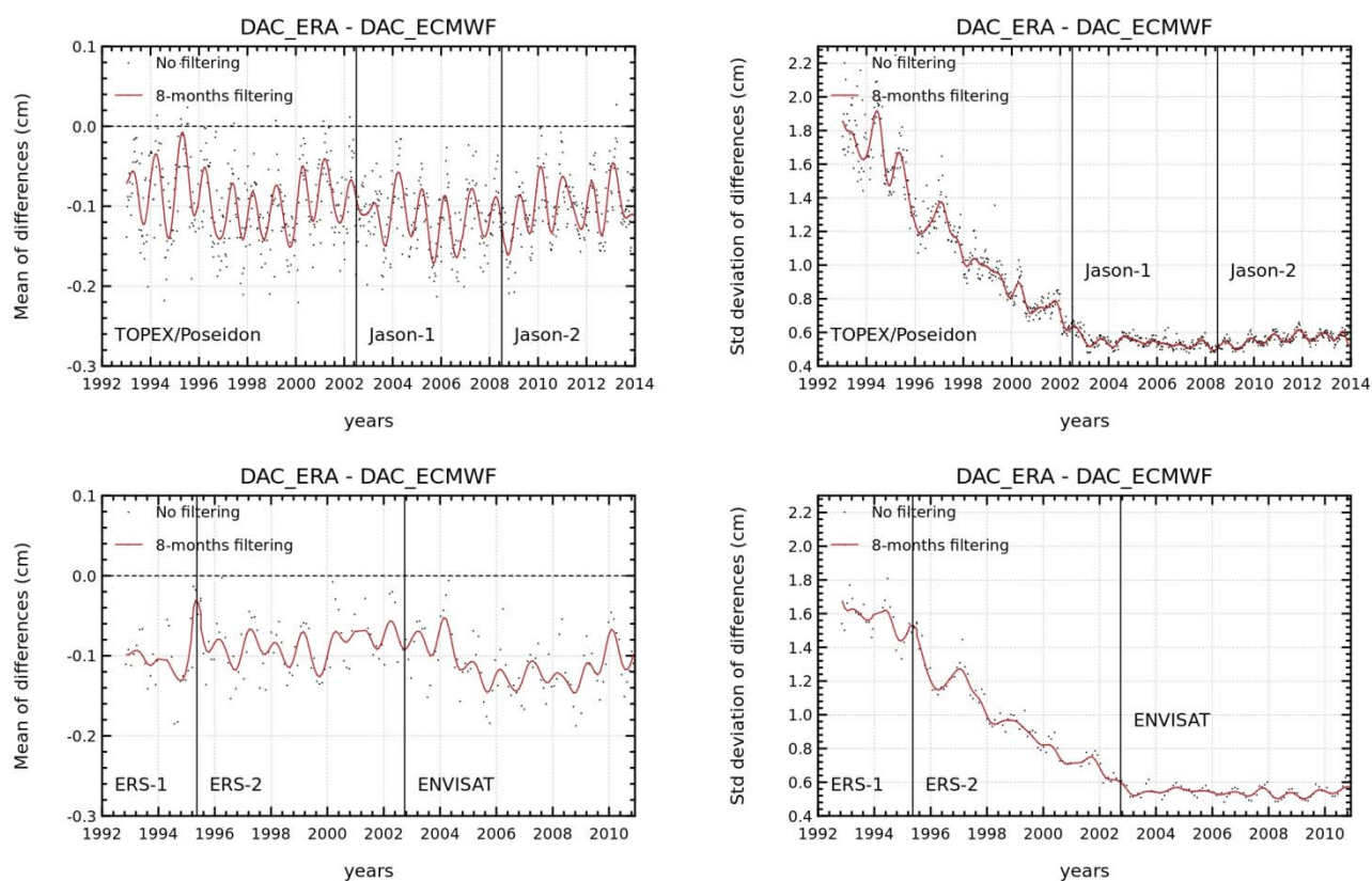
Figure 3: Temporal evolution of the global differences between DAC_ERA and the operational DAC seen by each altimeter missions : TP, Jason-1 and Jason-2 above and, ERS-1, ERS-2, Envisat below (mean and standard deviation in cm).
