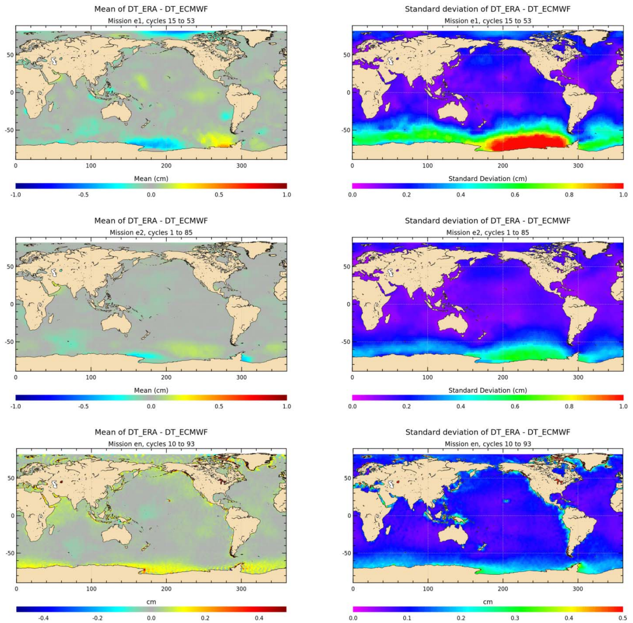
Figure 6 : Maps of differences between DT_ERA and the ECMWF operational DT seen by altimetry missions ERS-1, ERS-2 and Envisat (mean and standard deviation in cm).
