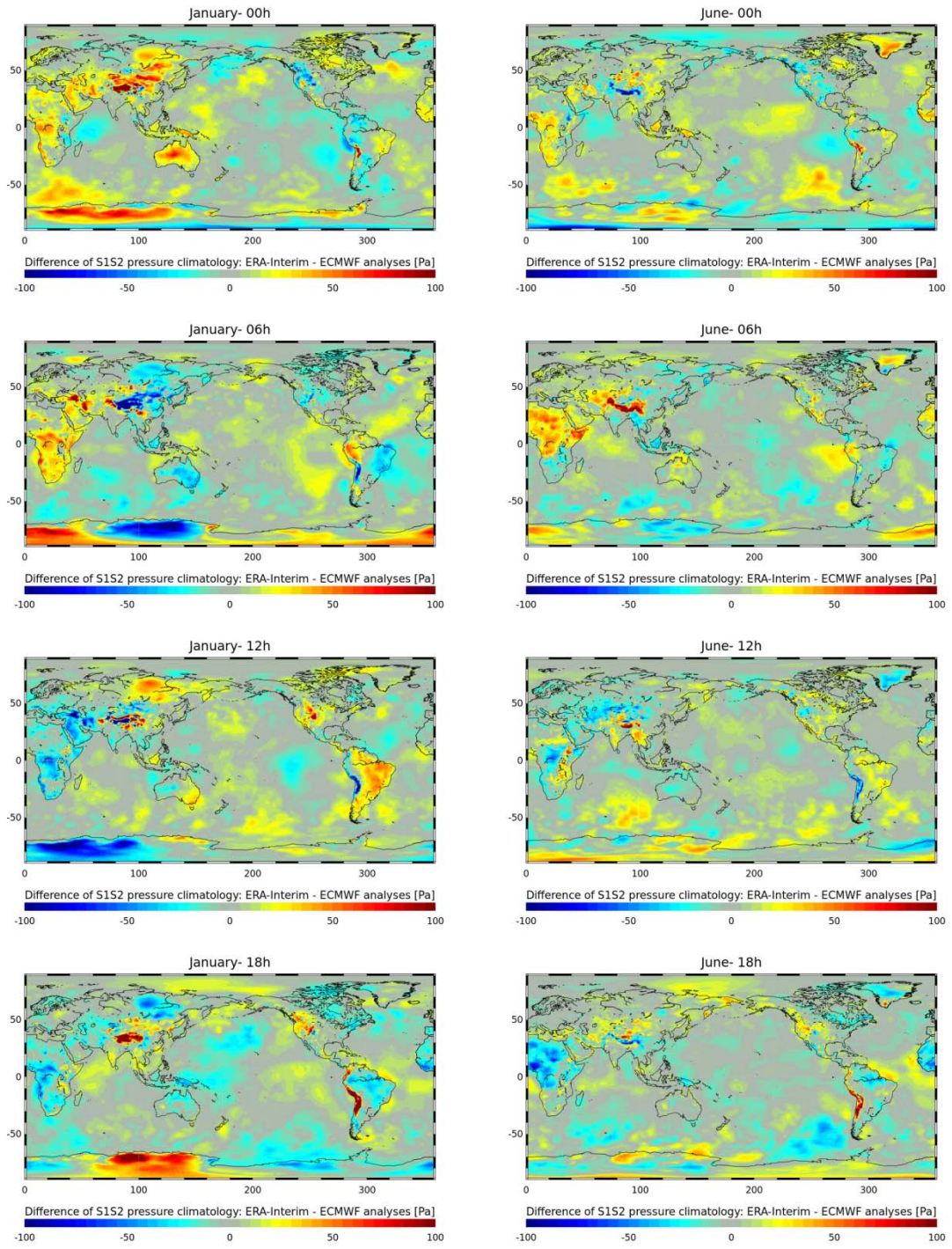
Figure 2: Difference of S1S2 atmospheric pressure climatologies from ERA-Interim and ECMWF analyses, where S1 and S2 respectively represent the diurnal and semi-diurnal atmospheric tides.
