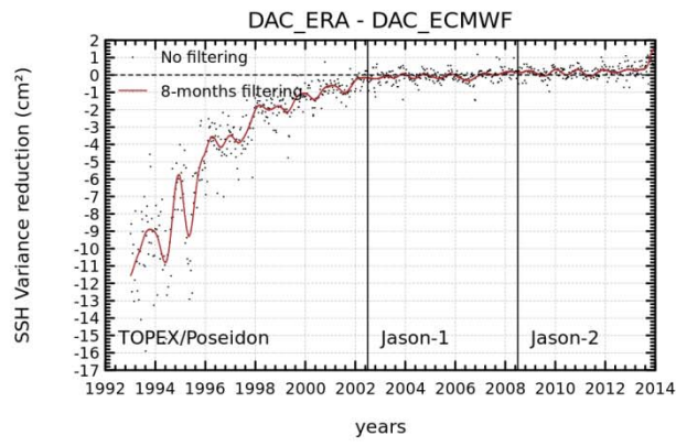
Figure 7: Temporal evolution of SSH variance differences at crossovers using successively the ERA-Interim and reference DAC solutions in the SSH calculation for TOPEX/Jason-1/Jason-2 time series (on left), and ERS-1/ERS-2/Envisat time series (on right).
