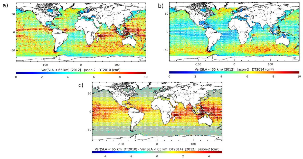
Figure 4 : Variance of the short wavelength signal removed (by low-pass filtering) on L3 along-track J2 SLA in the DT2010 (a) and DT2014 (b) versions. c) Difference between a) and b). Statistics done over year 2012.
