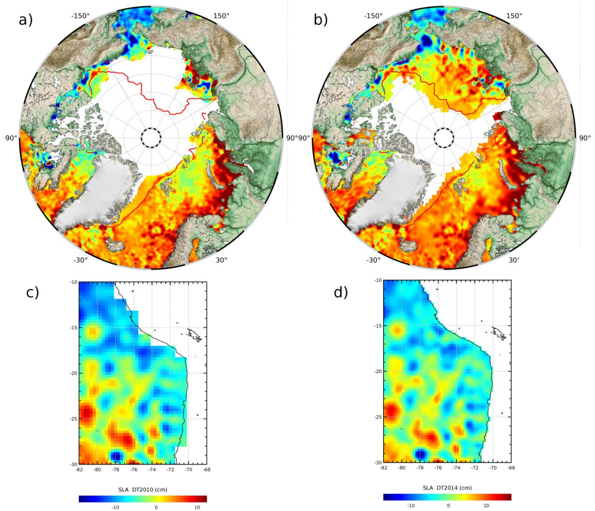
Figure 7: Coverage improvement associated with the DT2014 reprocessing. Map of SLA for day 2011/10/17 over the Arctic Ocean observed with the DT2010 (a) and DT2014 (b) products. Sea ice extent is shown with red line (OSISAF product). Same map along the western South American coast with DT2010 (c) and DT2014 (d).
