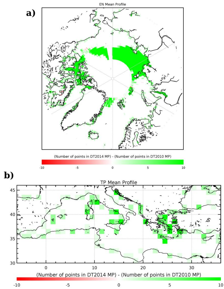
Figure 3: Differences of the number of points defined along the DT2014 and DT2010 versions of the Mean Profile defined along theoretical EN (a) and TP (b) tracks. Statistics done in 1^\circ \times 1^\circ boxes.
