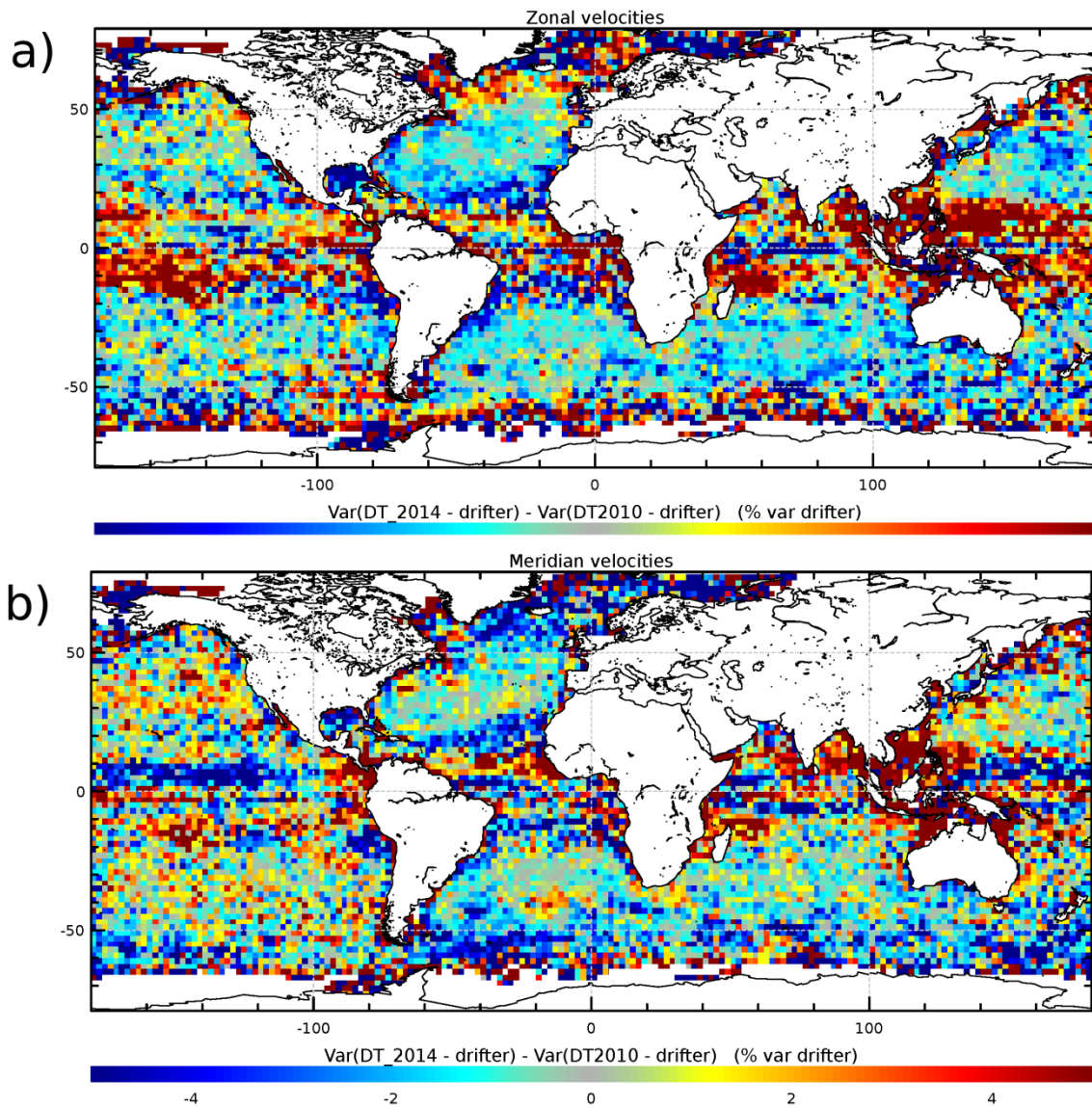
Figure 12: Maps of the difference of the variances of the altimeter geostrophic currents minus drifter measurement differences, using successively DT2014 and DT2010 SLA gridded products. The difference of variance is expressed in % of the drifter variance. Zonal (a) and meridional (b) component differences. Negative values mean that the variance of the differences between geostrophic currents from altimetry and from drifter measurement is reduced when considering the DT2014 product.
