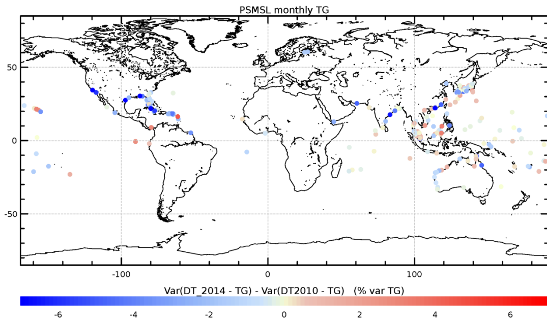
Figure 13: Difference of the variance of the altimeter SLA minus tide gauge SLA differences, using successively DT2014 and DT2010 SLA gridded products. Monthly TG from PSMSL. Negative values mean that the SLA differences between altimetry and tide gauges is reduced when considering DT2014 products.
