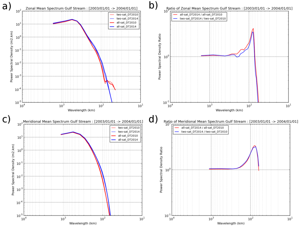
Figure 8: Mean zonal (a) and meridional (c) power spectral density (PSD) computed from gridded DT2014 (blue) and DT2010 (red) all-sat-merged (UPD; thick line) and two-sat-merged (REF; thin line) SLA fields over the Gulf Stream area during 2003 (when the constellation included J1, TP Tandem, Geosat Follow On and EN). Ratio between DT2010 and DT2014 PSD when all-sat-merged (UPD; red line) and two-sat-merged (REF; blue line) are considered: zonal (b) and meridional (d) components.
