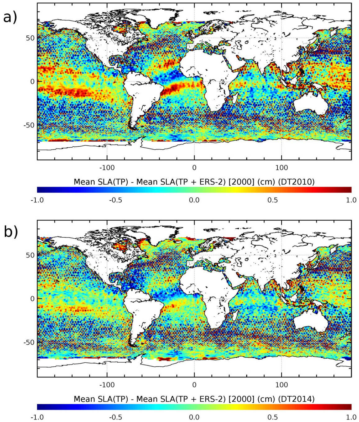
Figure 15: Difference of the mean SLA over the year 2000, measured with TP only, and with the merged TP+ERS-2 product. Comparison done for the DT2010 (a) and DT2014 (b) products.
