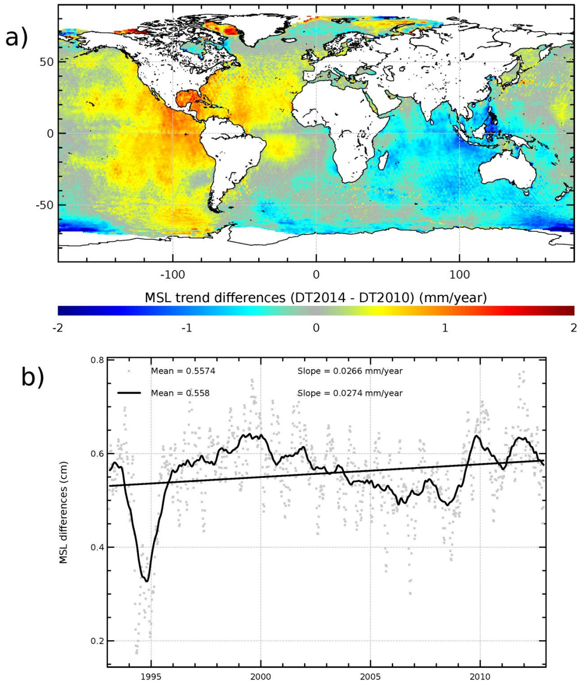
Figure 14: a) Map of the differences of the local MSL trend estimated from the DT2014 and DT2010 gridded SLA products. MSL estimated over the [1993, 2012] period. b) Temporal evolution of the differences of the global MSL estimated from DT2014 and DT2010.
