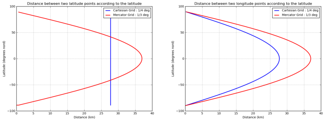
Figure C1 : Left : Difference between two successive grid points on a meridional section as a function of latitude, at 1/4^\circ \times 1/4^\circ Cartesian resolution (blue) and 1/3^\circ \times 1/3^\circ Mercator resolution (red). Right: same as left but for a zonal section.
