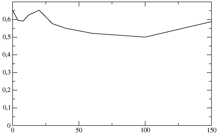
Figure 2 : RMS error on temperature, after a filter analysis, given a length of the localisation. The table below gives the correspondance between the length numbers and the localisation in degrees.
