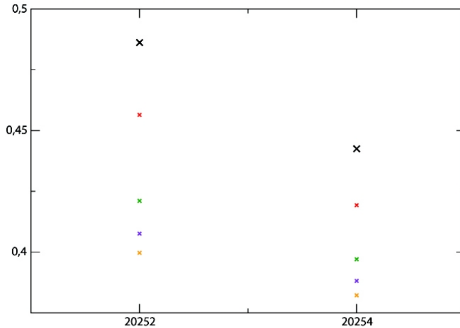
Figure 1 : RMS error on temperature (on the whole domain), after the filter analysis (black), and the smoother analyses with : 2 (red), 6 (green), 10 (purple) or 16 (orange) days retrospective assimilations.
