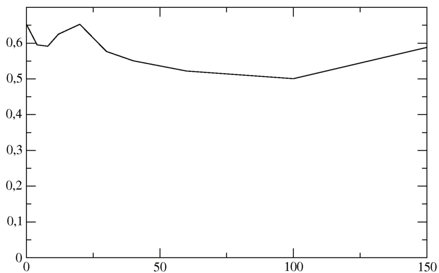
Fig. 2. RMS error on temperature, after a filter analysis, given a length of the localisation. The table below gives the correspondance between the length numbers and the localisation in degrees.
