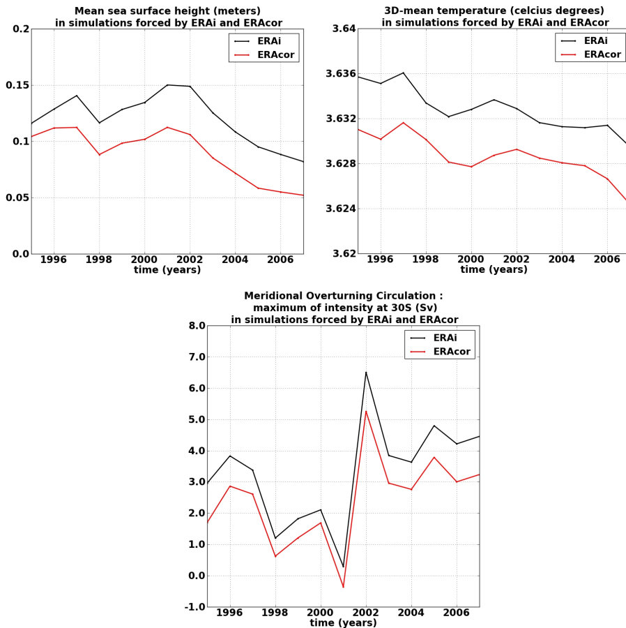
Fig. 11. Comparison between the simulations forced by ERAi (black) and ERAcor (red). Top: time-series between 1995 and 2007 of the global mean of the sea surface height in m (left), and of the global mean of the temperature in ^{\circ}C (right). Bottom: time-series between 1995 and 2007 of the maximum intensity of the meridional overturning circulation at 30S in Sv .
