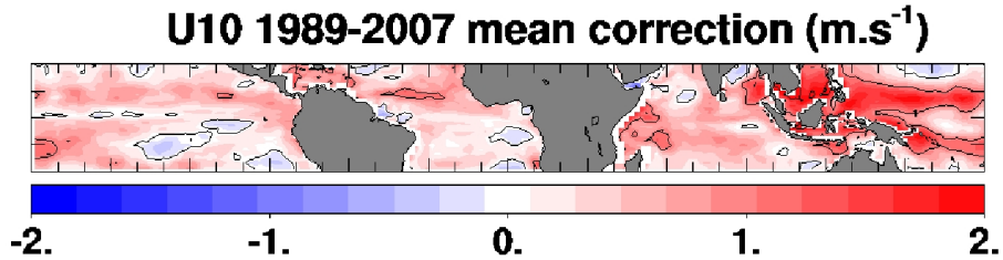
Fig. 8. 1989-2007 mean wind speed correction in the 20N-20S latitude band. Isocontours from -2 to 2 m.s^{-1} by 1.
