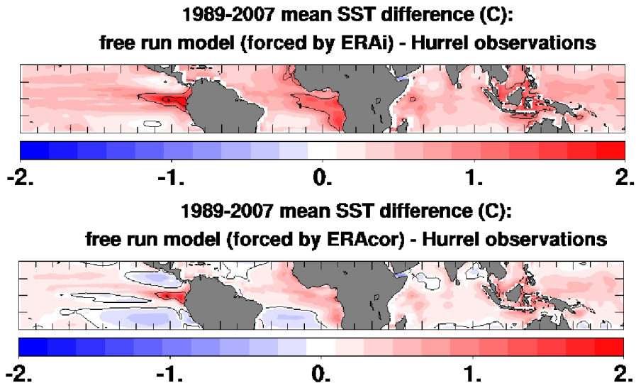
Fig. 10. 1989-2007 mean differences between Hurrell SST and free model run forced by ERAi (top), and between Hurrell SST and free model run forced by ERAcor (bottom) in the 20N-20S latitude band.
