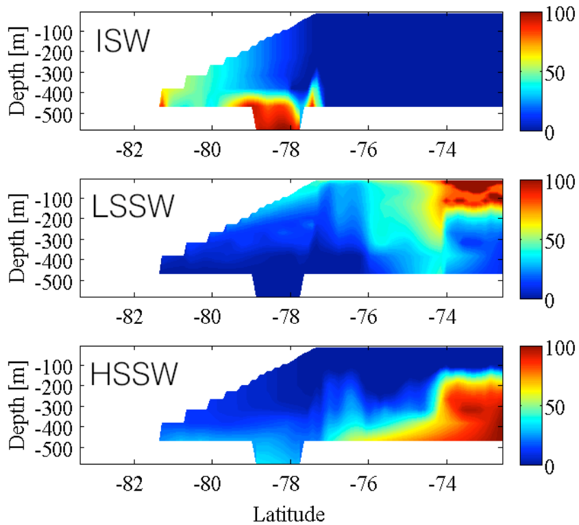
Fig. 4. Water masses spacial contribution (%) over de continental shelf at the meridional section along the 175°E from modeled data. Ice Shelf Water (ISW); Low Salinity Shelf Water (LSSW) and High Salinity Sh
