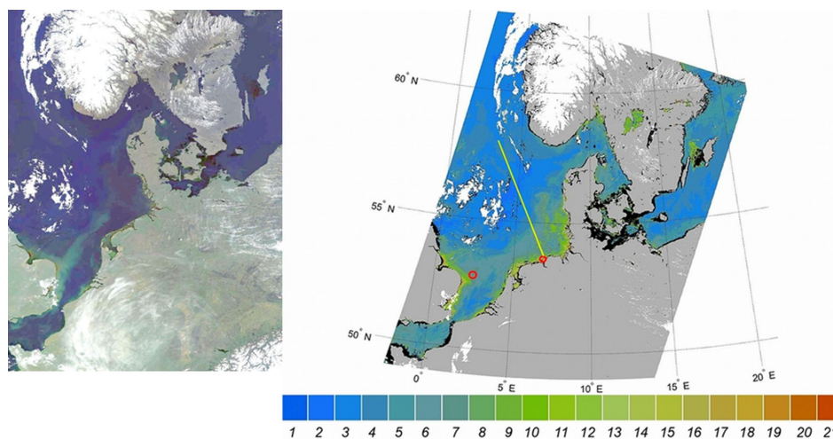
Fig. 1. Fig. 5. Left. MERIS true colour image (4 May 2006). Right: The spring FU map of the turbid North Sea of shows FU values ranging from 3 to 9 (red circle near England FU6). The Wadden Sea area within bar
