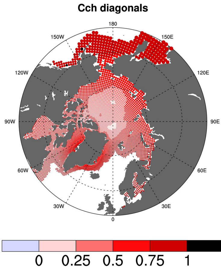
Fig. 2. Correlation between sea-ice concentration and mean sea-ice thickness at the same grid point diagnosed from a long model run with Eq.~(24) of the manuscript.
