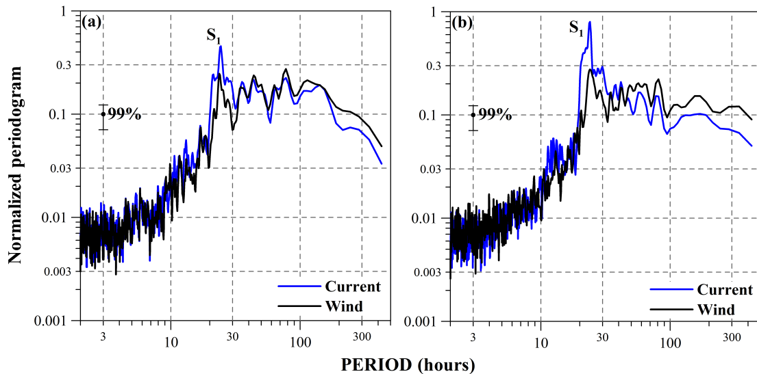
Fig. 3. Fig. 7. Normalised Lomb-Scargle periodograms (99% confidence level) for: (a) the first and (b) the second canonical variables of the currents (blue) and winds (black).
