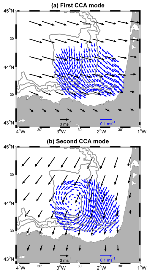
Fig. 1. Fig. 5. Maps of homogeneous regression coefficients (m/s) (significant at the 95% confidence level) of the: (a) first and (b) second CCA modes for the currents (blue) and winds (black) at D1 domain.
