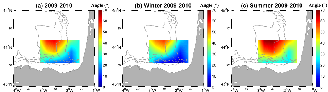
Fig. 2. Fig. 6. Deflection angles of the wind-induced surface flows for the first CCA mode in: (a) 2009-2010, (b) wintertime (October-March) 2009-2010 and (c) summertime (April to September) 2009-2010 periods
