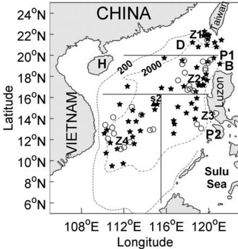
Fig. 5. Four geographic zones of SCS, adopted from Wang et al. (2003) Circles denote cyclonic eddies, and stars anticyclonic eddies.
