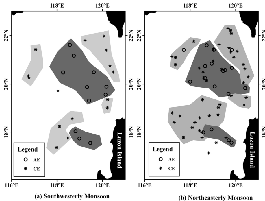
Fig. 9. Eddies of A1 and C1 generated in Northeastern SCS during different monsoon seasons. Concentration regions of AEs and CEs are generally represented by different colors.
