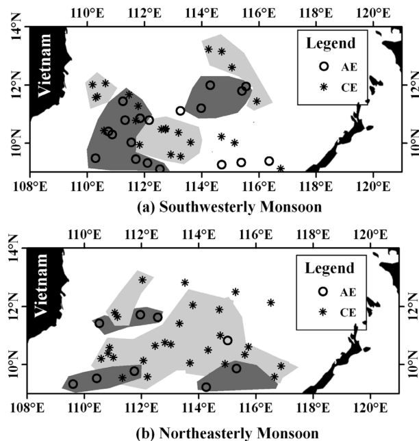
Fig. 10. Eddies of A8, A9, A10, C5 and C6 generated in Southern SCS during different monsoon seasons. Concentration regions of AEs and CEs are generally represented by different colors.
