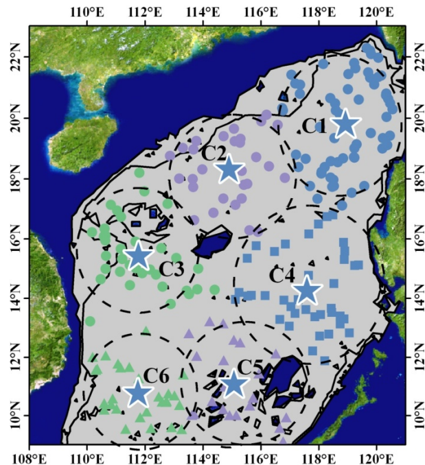
Fig. 7. Six-cluster result for cyclonic eddies. Blue stars are cluster centroids. Black dashed lines show approximate area of clusters. Different groups are distinguished by different colors or symbols.
