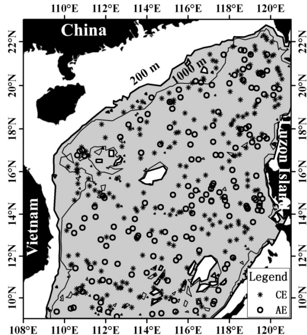
Fig. 1. Map of study area. Birth locations of cyclonic and anticyclonic eddies are symbolized by the asterisk and circle, respectively. Black solid lines indicate 200-m (bold) and 1000-m (thin) isobaths.
