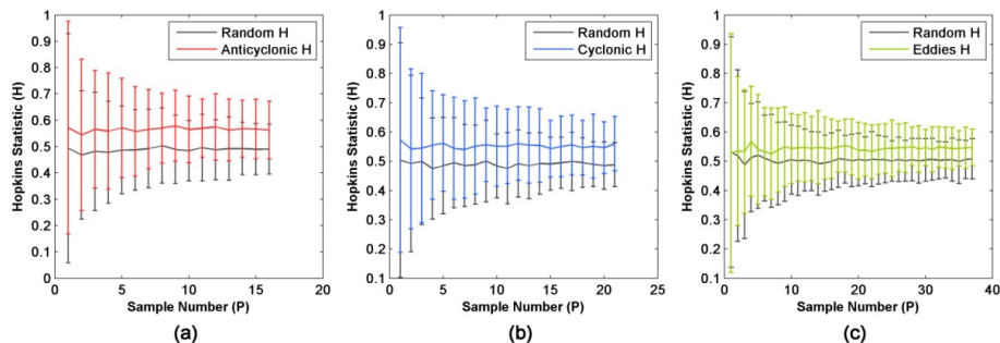
Fig. 2. Error bar plot of Hopkins statistic. Error bar is twice the standard deviation, and curve is mean of H. (a) Hopkins statistic of AE and random sample. (b) Hopkins statistics of CE and random sample. (c) Hopkins statistics of all eddies and random sample.
