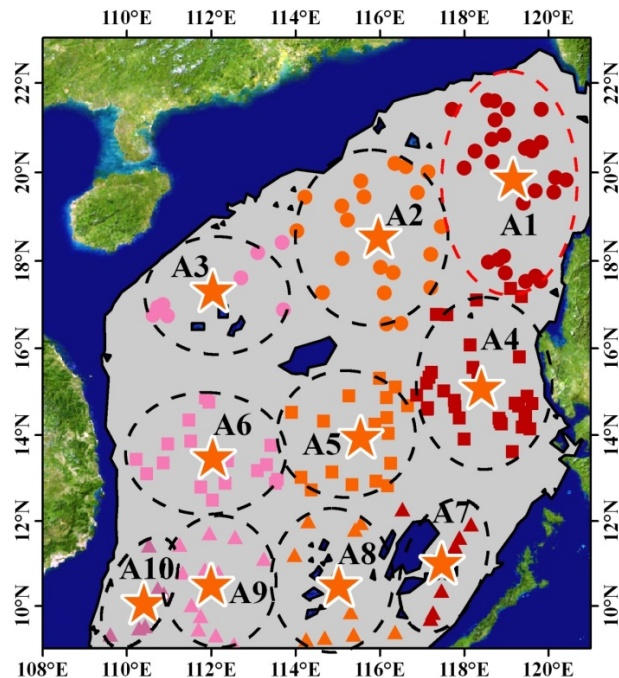
Fig. 6. Ten-cluster result for anticyclonic eddies. Orange stars are cluster centroids. Black dashed lines outline approximate area of clusters. Different groups are distinguished by different colors or symbols.
