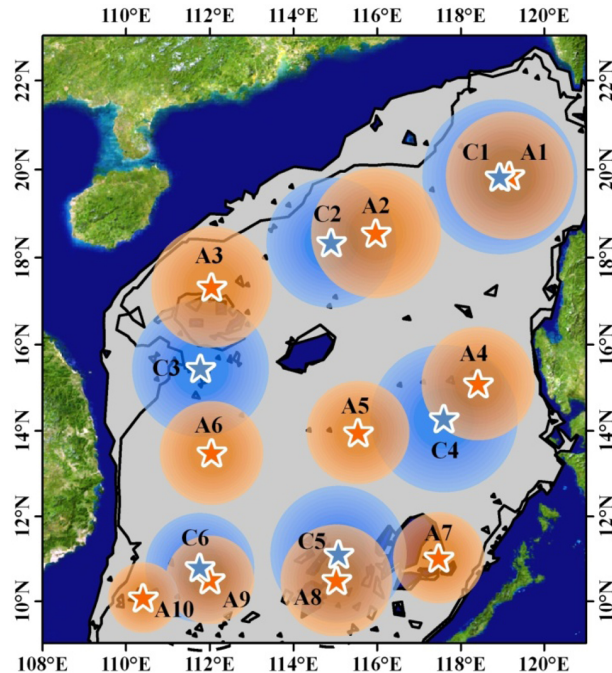
Fig. 8. Centroids and spatial domains of cyclonic and anticyclonic eddies. Centroids of AEs and CEs are shown by stars of different colors. The circles in different colors represent the spatial dimension of each cluster, and the radius is defined by the mean distance from these eddies' generation locations to corresponding centroid.
