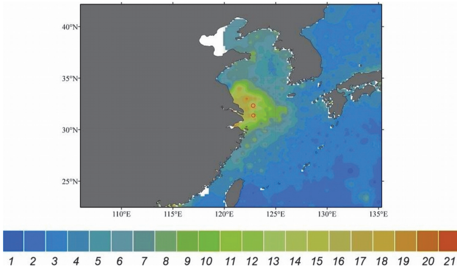
Fig. 12. Yellow Sea map based on 2882 FU in-situ observations collected during winter between 1930 and 1999. Within the red circles the colour is FU12 (lower, in front of the Yangtze outflow) and FU14 (upper). Near coast FU-numbers are as high as 18 to 20.
