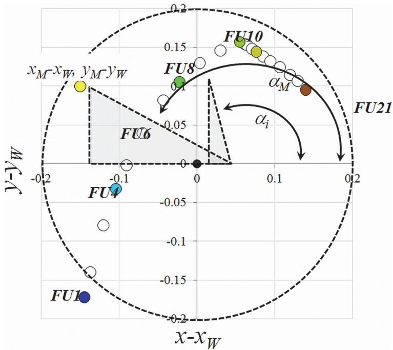
Fig. 3. Chromaticity diagram with scale colours FU1 to FU21 shown in dots, relative to the white point that is set at the origin. As an example the angle \alpha_i ( 102.05^\circ , see Table 3), determining the position of FU8, is given.
