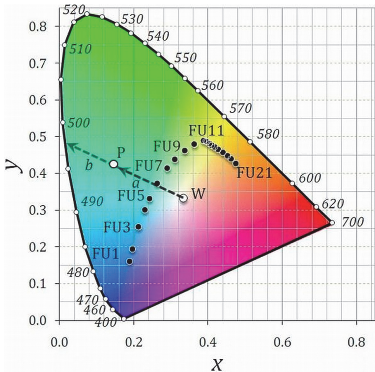
Fig. 2. The chromaticity coordinates, based upon transmission measurements, of the FU scale colours 1 to 21 (black circles) and the white point W where x_W = y_W = 1/3 . The outer curved boundary is the spectral locus, with the corresponding mono-chromatic wavelengths shown in nanometre.
