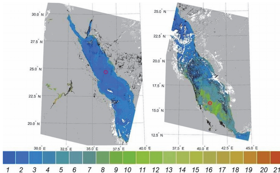
Fig. 6. The winter FU map of the Red Sea, dated 22 (left) and 23 December 2003 (right) shows that open water of the northern part is mainly bluish FU1 to FU2 (in red circle FU2) and near coast values are around FU3. The southern part shows more greenish coloured water (in red circle FU = 8).
