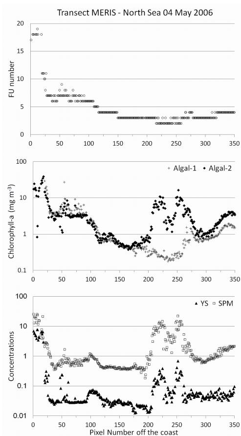
Fig. 9. Transect from the inner Wadden Sea to the Central North Sea. The upper panel shows the FU values, the middle panel the two MERIS products for chlorophyll a and the low panel shows the concentration of SPM (units in \text{g m}^{-3} ) and yellow substance (absorption in \text{m}^{-1} at 442 nm)
