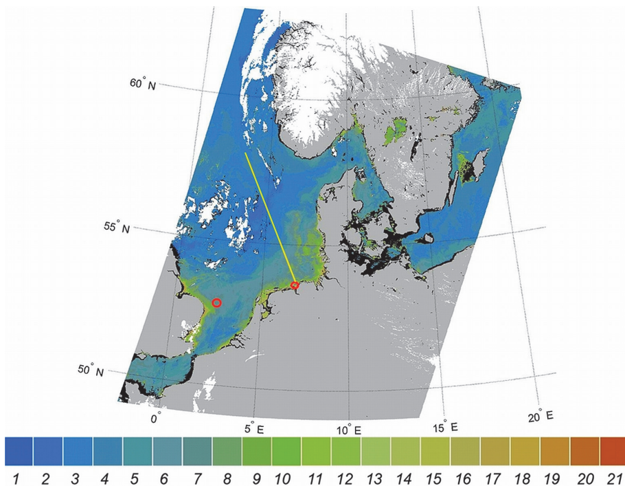
Fig. 5. The spring FU map of the turbid North Sea (4 May 2006) shows FU values ranging from 3 to 9 (red circle near England FU6). The Wadden Sea area within barrier islands north of Holland shows values between FU9 and FU18. The area within the red circle indicates a pixel value of FU = 14. The yellow line shows the transect extracted from the MERIS image and shown in Fig. 9.
