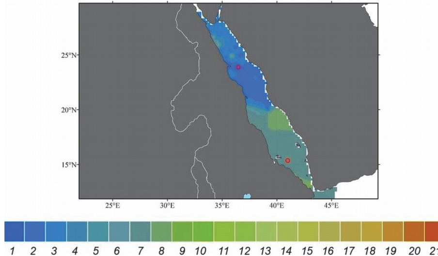
Fig. 11. The Red Sea map based on 52 FU in-situ observations collected during the winters of 1895 to 1898. Within the northern red circle FU = 2 and within the southern red circle FU = 7 . This colour boundary can also be observed 100 yr later in the MERIS map of 6.
