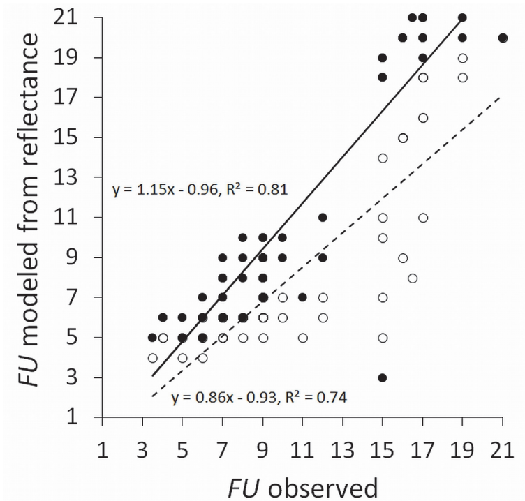
Fig. 10. Scatterplot of the FU numbers modelled using full reflectance spectra (black dots) with trend line (full) and from the reflectance at MERIS bands (circles) with trend line (intermittent) versus in situ observed FU numbers.
