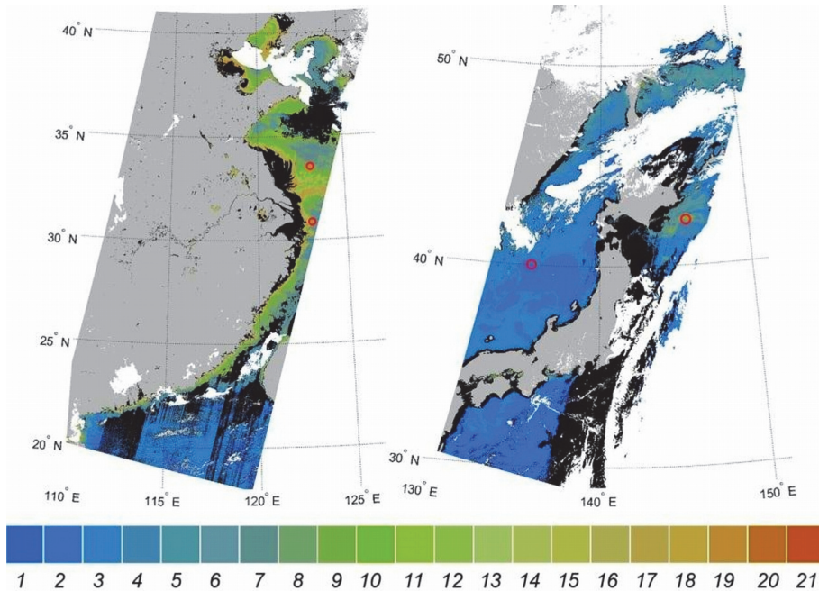
Fig. 7. The winter FU map of the Yellow Sea, acquisition date 11 February 2009 (left) and the summer FU map of the Sea of Japan, acquisition date 14 June 2004 (right). The Yellow Sea is mainly greenish brown with FU7 up to FU17 (FU9 in the lower red circle and FU11 in the upper red circle). The Sea of Japan, a “blue sea”, shows summer values of around FU2 to FU3 (in red circle FU2). East of Hokkaido phytoplankton abundance greens the water to FU10 (FU9 within the red circle east).
