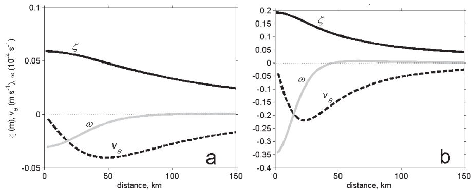
Fig. 5. Radial profiles of \zeta (m, solid black line), v_\theta ( \text{m s}^{-1} , dash line) and \omega ( 10^{-4} \text{ s}^{-1} , solid grey line) of the surface signal of a meddy with R_m = 30 \text{ km} , H = 1100 \text{ m} and |\tilde{q}_m| = 0.7f ; (a) in the northern subtropics, (b) in the southern subtropics.
