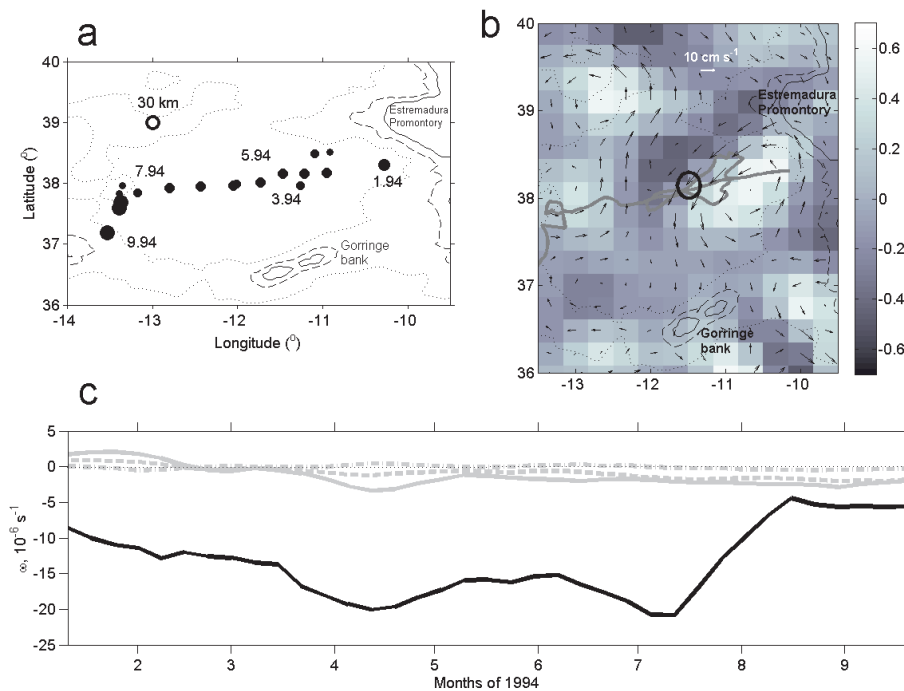
Fig. 3. Same as Fig. 1, but for the meddy Pinball; (b) shows the AVISO derived currents on 4 May 1994.
