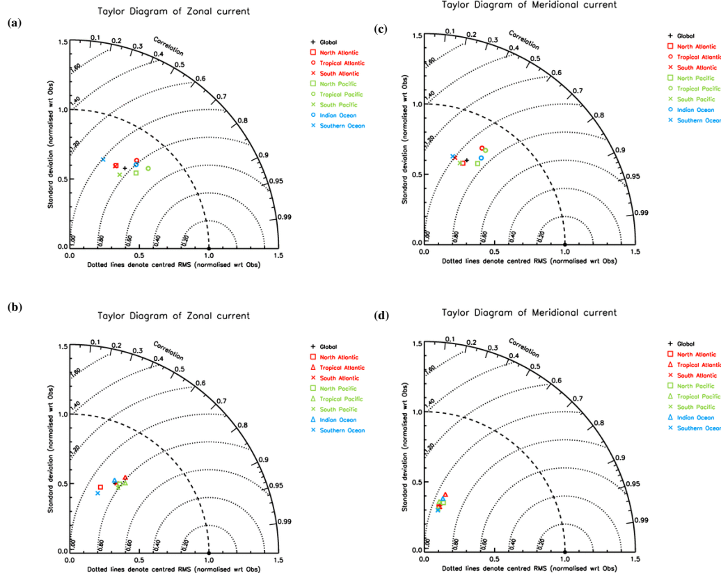
Fig. 3. Taylor plots showing the global drifter current validation for the FOAM V1 hindcast run (a) and for the drifter climatology (b) for zonal velocity. Corresponding Taylor plots for meridional velocity can be found in (c) and (d) . Results are shown for the whole global ocean as well as the same sub-basin areas used in Table 2.
