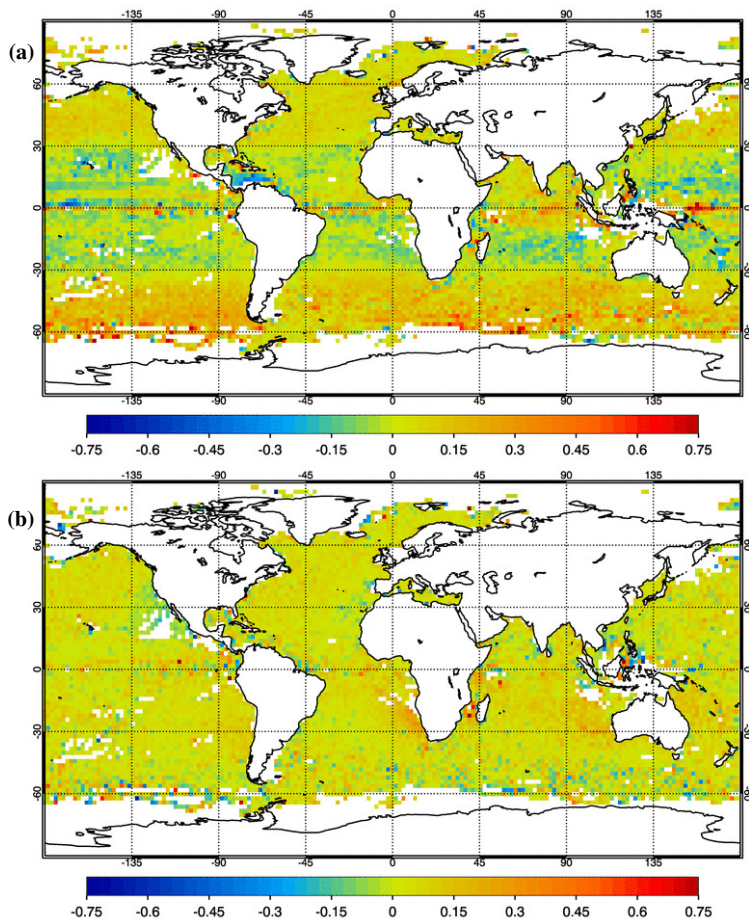
Fig. 4. Mean error (observed-modelled) against drifters for (a) zonal velocity and (b) meridional velocity in 2° bins.
