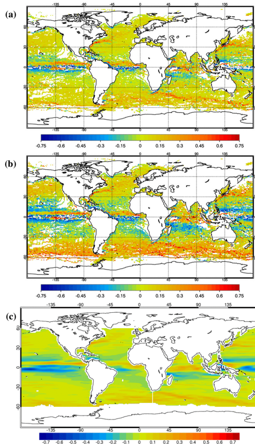
Fig. 5. Average zonal velocity fields over the 2007–08 study period in 1^\circ bins: (a) FOAM model values and (b) drifter-derived observation values at observation points. The corresponding averaged OSCAR zonal velocity is shown in (c) .
