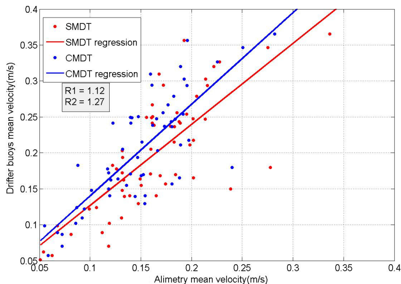
Fig. 1. Fig. 8. Scattergram of mean amplitudes of drifting buoys and altimetric velocities, reconstructed using SMDT and CMDT.
