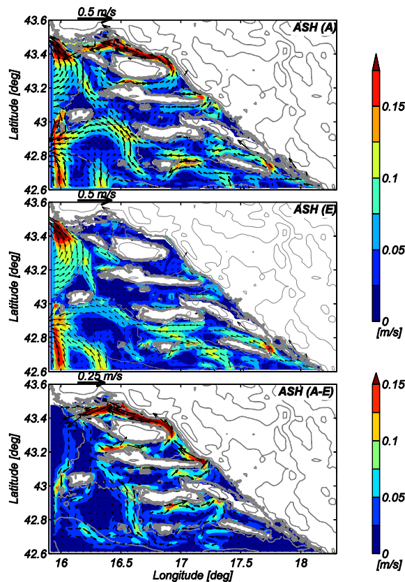
Fig. 4. The mean ASHELF-2 modeled vertically averaged currents for the B2 Bora period (Table 1) obtained with ALADIN and ECMWF forcing (top and center, respectively) and the differences between these two (bottom panel). Additionally, the magnitudes of vector differences |\text{ALADIN} - \text{ECMWF}| are shown in colors.
