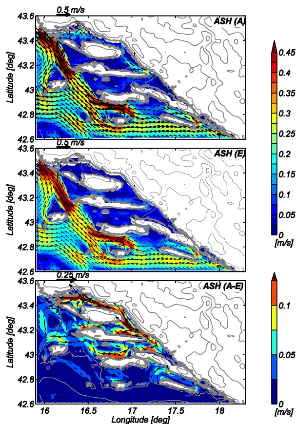
Fig. 7. The mean ASHELF-2 modeled vertically averaged currents for the Sirocco episode (Table 1) obtained with ALADIN and ECMWF forcing (top and center, respectively) and the differences between these two (bottom panel). Additionally, the magnitudes of vector differences |\text{ALADIN} - \text{ECMWF}| are shown in colors.
