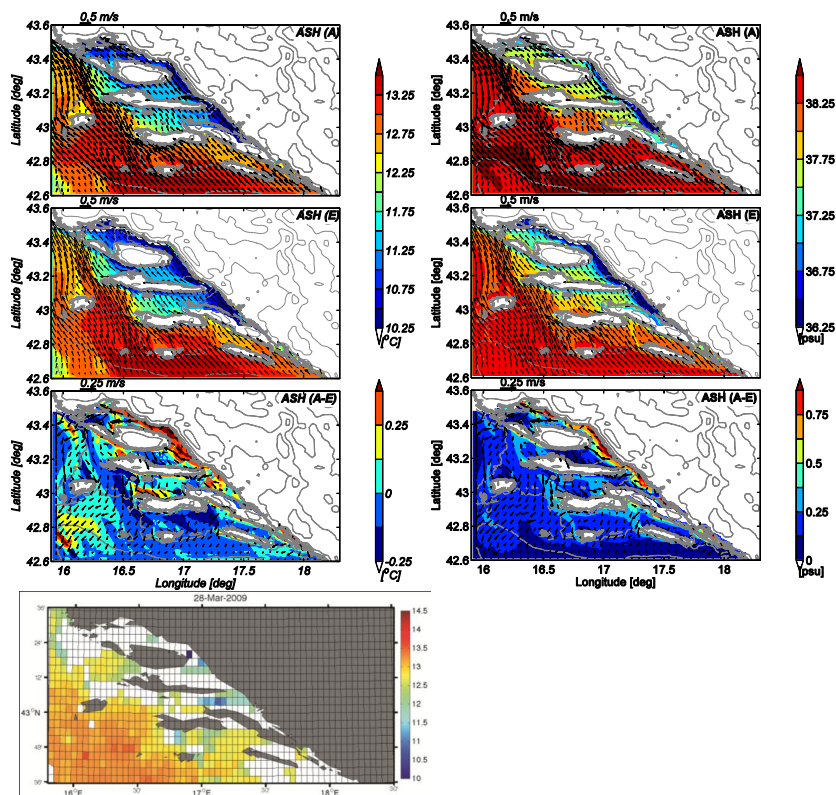
Fig. 8. Mean ASHELF-2 modeled surface temperatures (left) and surface salinities (right panels) for the Sirocco period (Table 1) obtained with ALADIN (top) and ECMWF (second from above) forcing and the differences between these two (third from above). Vectors show modeled surface currents and differences in surface currents (upper two rows and the third row, respectively). The lowermost panel shows the satellite-measured sea surface temperature for 28 March 2009.
