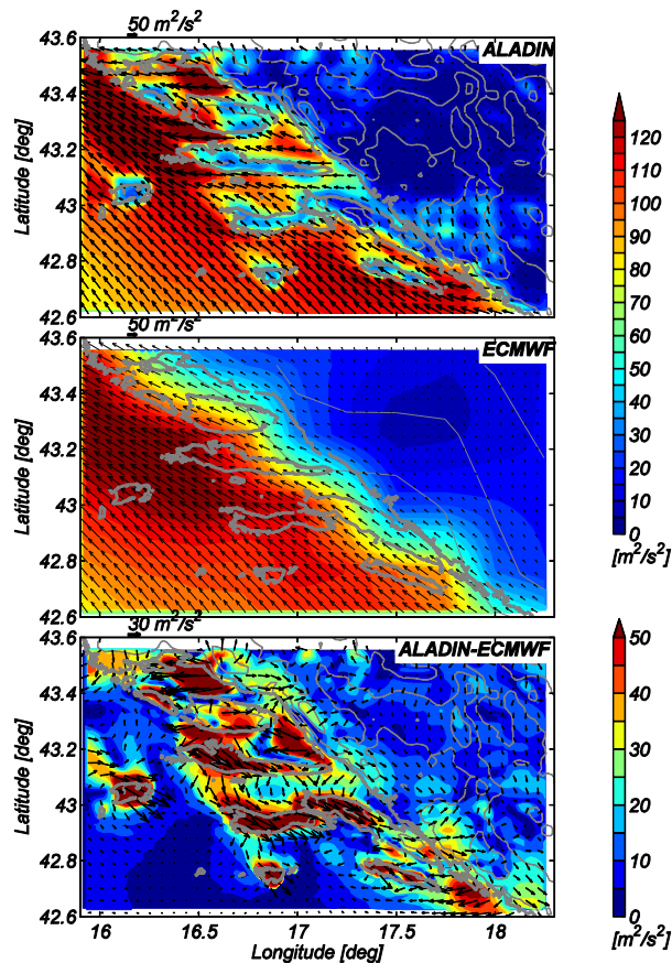
Fig. 6. Mean ALADIN (top) and ECMWF (center) modeled pseudo-stress for the Sirocco episode (Table 1). The bottom panel shows the difference between these two. Topography contours, as seen from the models, and shore lines are indicated by thin and thick gray lines, respectively.
