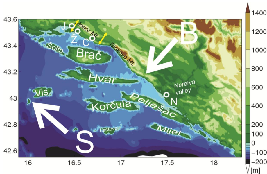
Fig. 1. Modeling domain and the actual topography. Positions of the two mountain passes (one northwest and the other southeast of Mosor Mountain) are indicated in yellow. The white circles show river estuaries for Jadro (J), Žrnovnica (Ž), Cetina (C) and Neretva (N). Large white arrows indicate general Bora (B) and Sirocco (S) wind directions.
