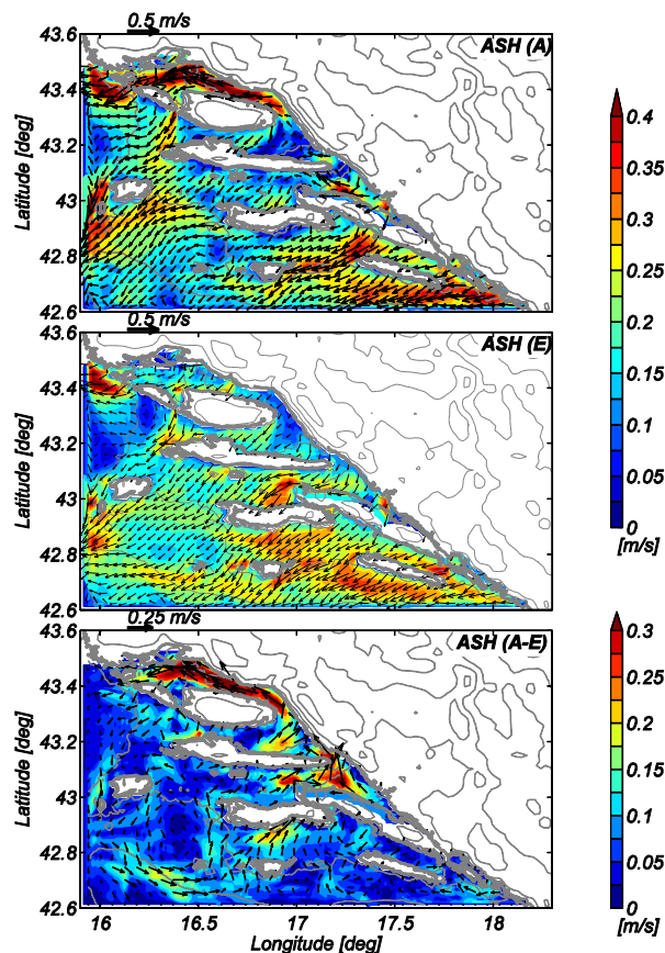
Fig. 3. The ASHELF-2 modeled mean surface currents for the B2 Bora period (Table 1) obtained by ALADIN and ECMWF forcing (top and center, respectively) and the differences between these two. Additionally, the magnitudes of vector differences |\text{ALADIN} - \text{ECMWF}| are shown in colors.
