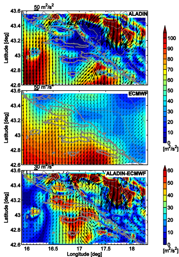
Fig. 2. Mean ALADIN (top) and ECMWF (center) modeled wind pseudo-stress for the B2 Bora episode (Table 1). The bottom panel shows the difference between these two. Additionally, the magnitudes of vector differences |\text{ALADIN} - \text{ECMWF}| are shown in colors. Topography contours, as seen from the models, and shore lines are indicated with thin and thick grey lines, respectively.
