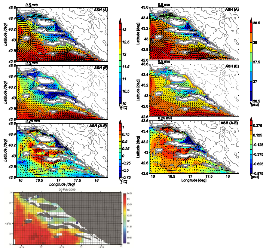
Fig. 5. Mean ASHELF-2 modeled surface temperatures (left) and surface salinities (right panels) for the B2 Bora period (Table 1) obtained by ALADIN and ECMWF forcing (upper two rows) and the differences between these two (third row). Vectors show surface currents and differences in surface currents (upper two rows and the third row, respectively). The lowermost panel shows the satellite-measured sea surface temperature for 20 February 2009.
