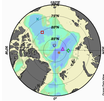
Fig. 17. Deep and bottom water characteristics from the Nansen Basin, Amundsen Basin, Makarov Basin and Canada Basin. Note the absence of a deep temperature minimum in the Makarov Basin and that the temperature minimum observed in the Canada Basin could derive from the Makarov Basin and the deep salinity maximum in the Amundsen Basin could be caused by Makarov Basin deep water crossing the Lomonosov Ridge.
