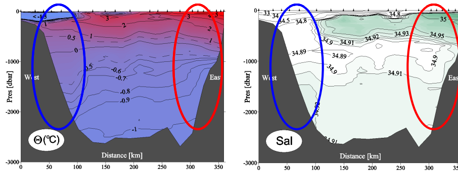
Fig. 20. Potential temperature and salinity sections from Fram Strait taken in 1997 by R/V Lance . The West Spitsbergen Current and the East Greenland Current are indicated by red and blue ellipses, respectively.
