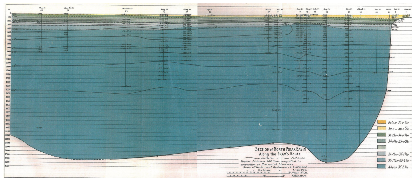
Fig. 2. Upper panel, map of the Arctic Ocean showing the drift of Fram and the track of Nansen and Johansen, map by Nansen, reproduced in Hayes (2003). Lower panel: temperature and salinity section based on the hydrographic observations made from Fram during the drift from the Laptev Sea to Fram Strait. From Nansen (1902).
