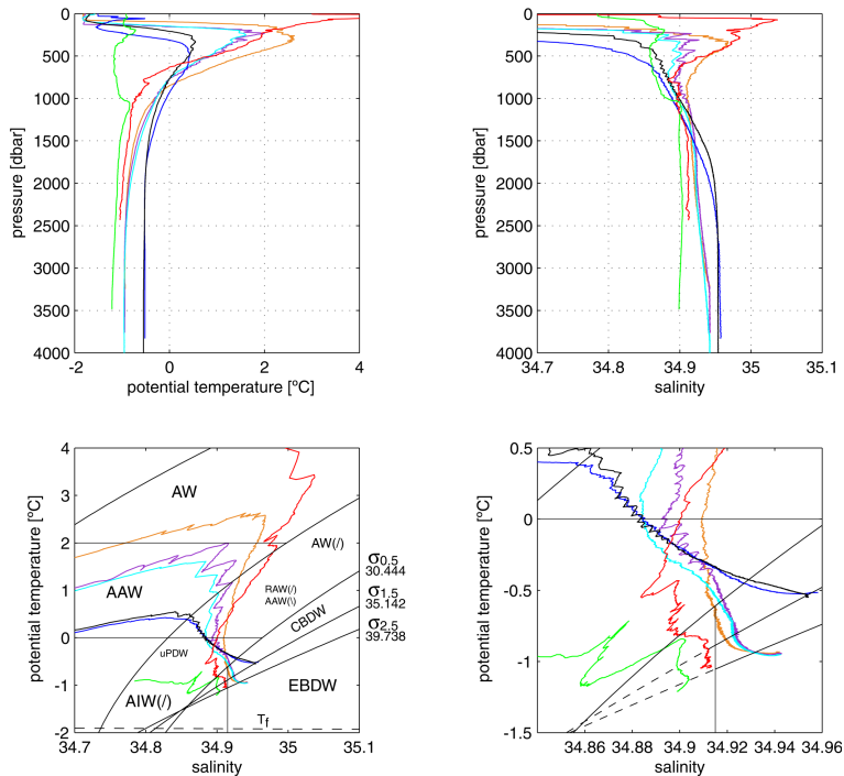
Fig. 10. Potential temperature and salinity profiles and TS curves showing the characteristics of some water masses in the Arctic Mediterranean. Green station, Greenland Sea, red station, Fram Strait, orange station, Nansen Basin slope, magenta station, Gakkel Ridge, cyan station, Amundsen Basin, black station, Makarov Basin, blue station Canada Basin. AW (Atlantic Water) AAW (Arctic Atlantic Water), RAW (Recirculating Atlantic Water), uPDW (upper Polar Deep Water) AIW (Arctic Intermediate Water), CBDW (Canadian Basin Deep Water) EBDW (Eurasian Basin Deep Water) NDW (Nordic Seas Deep Water) (/) indicates unstable stratification in either temperature or salinity (\) indicates stable stratification in both components. From Rudels (2009).
