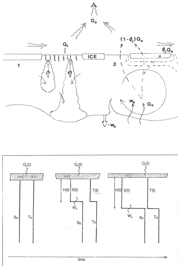
Fig. 5. Upper panel: schematics showing oceanic heat loss under freezing conditions and in the presence of sea ice (from Rudels, 1995). Lower panel: the evolution of the upper layer when warm water encounters sea ice under freezing conditions (from Rudels et al., 1999a).
