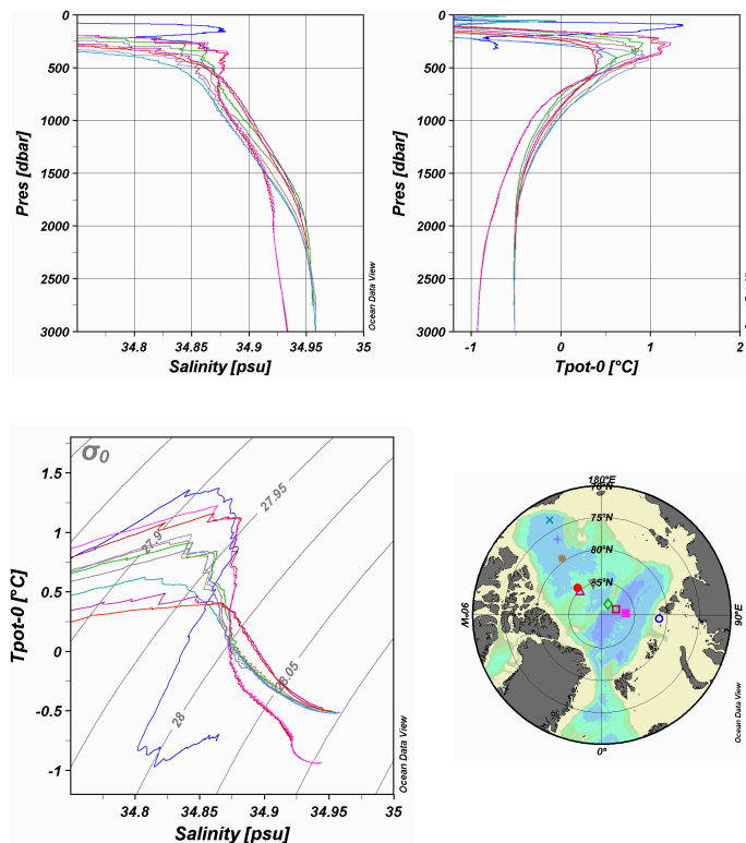
Fig. 14. Potential temperature and salinity profiles and TS curves comparing the Barents Sea branch characteristics with those found in the other basins. The Barents Sea branch could, at least theoretically, supply the Atlantic and intermediate water to the Arctic Ocean Basins beyond the Nansen Basin and the Gakkel Ridge. Data from Polarstern 2007 and Oden 2005.
