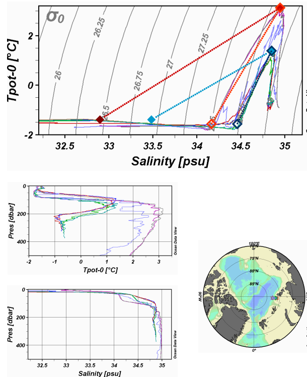
Fig. 7. Potential temperature and salinity profiles and TS diagrams showing the difference of the winter mixed layers and the Atlantic cores of the Fram Strait branch (red) and the Barents Sea branch (blue). In spite of having a cooler and less saline Atlantic layer the winter mixed layer of the Barents Sea branch, created by stirring melt water into the upper part of the Atlantic water, is more saline than that of the Fram Strait branch. The filled diamonds indicate the salinity of the mixed layer if all oceanic heat is going to ice melt, the open diamonds the salinity if minimum heat is going to ice melt based on the temperature and salinity of the Atlantic water.
