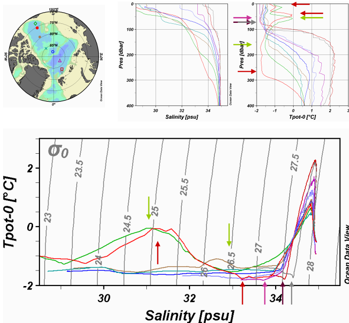
Fig. 8. Halocline features in the Arctic Ocean. The grey, dark red and magenta arrows indicate the temperature minimum created by the winter homogenization. The red arrows show on one station, the upper temperature maximum due to seasonal heating, the temperature maximum due to the inflow of Bering Strait Summer Water (BSSW) and a temperature minimum due to the presence of an (isolated?) eddy of Fram Strait branch lower halocline water. The Green arrows show the temperature maximum of the BSSW and the temperature minimum of the Bering Sea Winter Water (BSWW). Note that the BSWW is present also at the red upper seasonal temperature maximum on the green station and the temperature minimum of the winter homogenization is present above the BSSW maximum.
