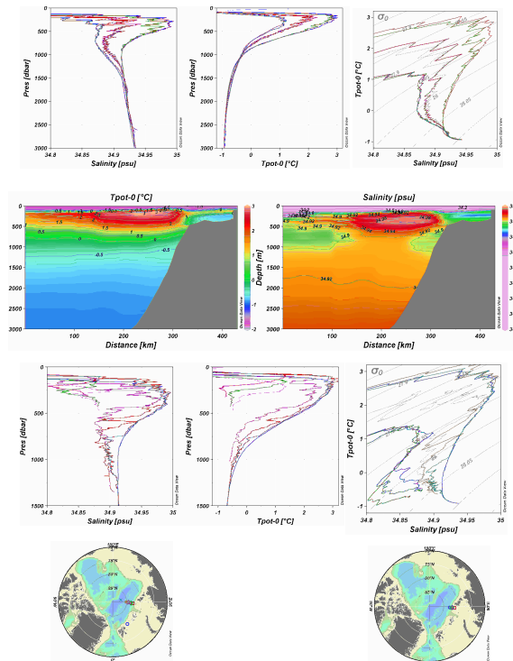
Fig. 12. Water masses mixing and interleaving in the Nansen Basin north of the Eastern Kara Sea. Central panel: temperature and salinity sections from the shelf to the Gakkel Ridge showing the warm saline Fram Strait Atlantic core and the cooler and less saline Barents Sea branch water on the slope and also on the basin side of the warm core. Upper panel: potential temperature and salinity profiles and TS curves from the deep basin showing the interleaving structures and different fronts. Lower panel: potential temperature and salinity profiles and TS curves from the slope showing the characteristics of the two branches and the mixing between them across the front. Data from Polarstern 2007.
