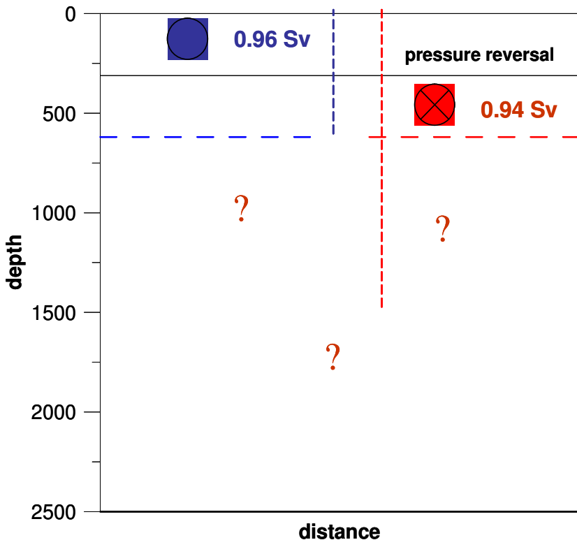
Fig. 21. Idealised baroclinic exchanges through Fram Strait, where the upper layer in the East Greenland Current is created by allowing 0.02 Sv of ice melt on the Atlantic water. The salinity of the low salinity layer, 34.27, is determined from the constraint that minimum heat goes to ice melt. The Atlantic water has temperature 3.1 and salinity 35. Only one pressure reversal is created and nothing, except the rise in sea level, will stop the inflow of Atlantic water and generate a barotropic component to the outflow.
