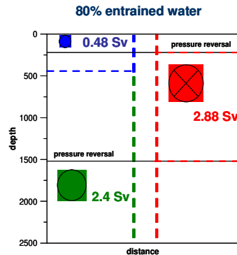
Fig. 22. Idealised baroclinic exchanges through Fram Strait. Half of the low salinity upper layer is assumed advected back on the shelves, where ice formation and brine rejection increase the salinity to 35 and the shelf water sinks down the slope entraining ambient (Atlantic) water. The increased density in the lower layer causes a second pressure reversal to form and a deep outflow is generated. However, the deep outflow does not cease, when mass balance is reached and the sea level in the Arctic Ocean will drop, adding a barotropic component to the Atlantic inflow to conserve mass.
