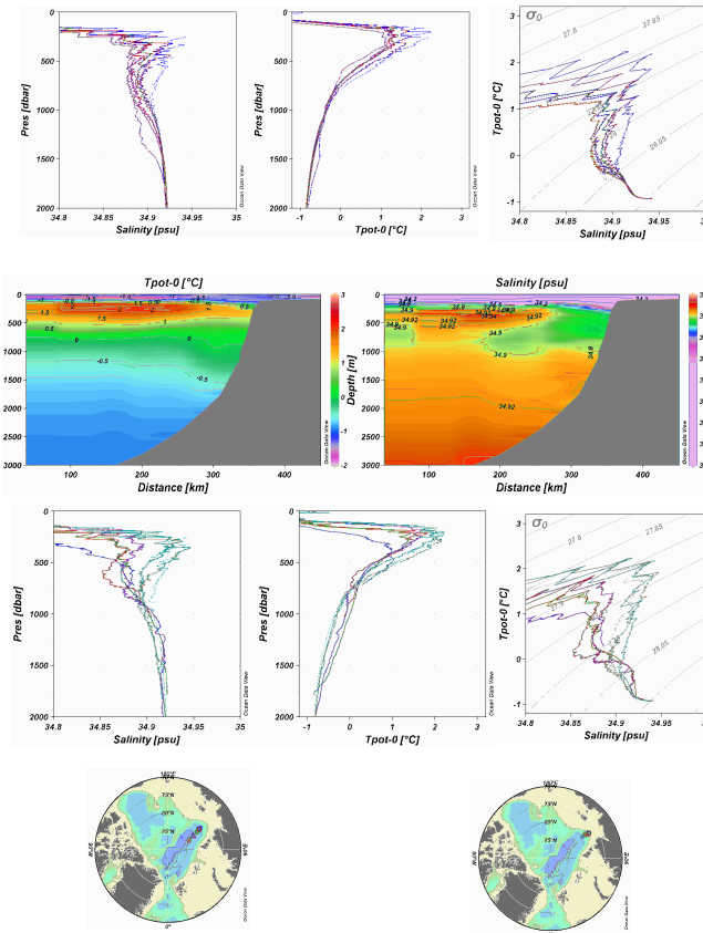
Fig. 13. Water masses mixing and interleaving along the Gakkel Ridge north of the Laptev Sea. Central panel: temperature and salinity sections from the shelf along the Gakkel Ridge showing a colder and less saline Fram Strait Atlantic core compared to the Kara Sea section (Fig. 12) and the Barents Sea branch water has spread from the slope into the basin. It is also on the basin side of the warm core. Upper panel: potential temperature and salinity profiles and TS curves from the deep basin showing the interleaving structures. Lower panel: potential temperature and salinity profiles and TS curves from the slope showing interleaving between the two branches. Note that no smooth warm and saline Atlantic core is present. Interleaving layers are found everywhere. Data from Polarstern 2007.
