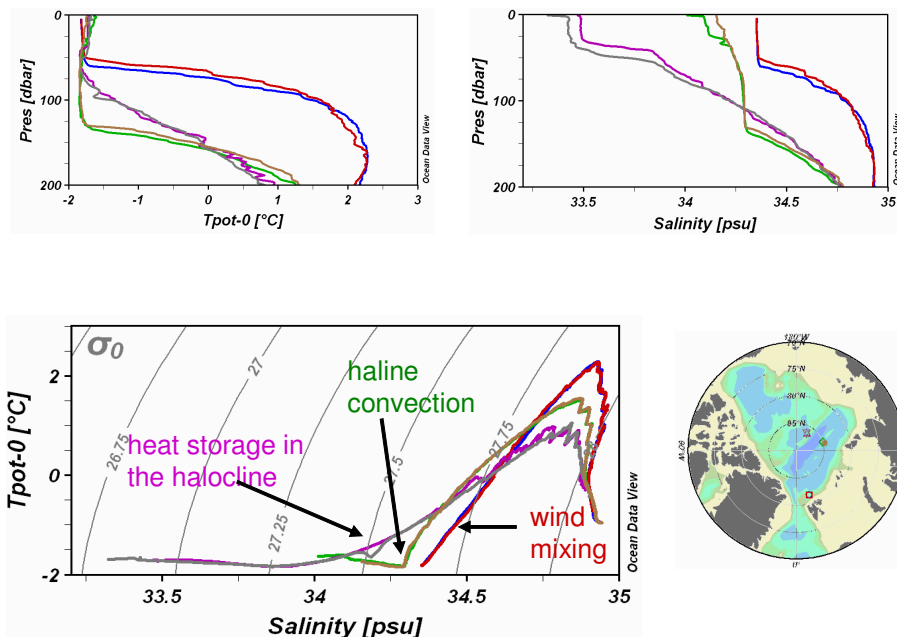
Fig. 6. Potential temperature and salinity profiles and TS curves from different parts of the Arctic Ocean showing the effects of wind mixing and heat entrained and lost to ice melt and to the atmosphere at the entrance to the Arctic Ocean, of haline convection bringing cold water into and cooling the thermocline in the Nansue Basin, and of heat mixed from below into and stored in halocline in the interior of the Arctic Ocean.
