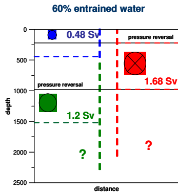
Fig. 22. Idealised baroclinic exchanges through Fram Strait. Half of the low salinity upper layer is assumed advected back on the shelves, where ice formation and brine rejection increase the salinity to 35 and the shelf water sinks down the slope entraining ambient (Atlantic) water. The increased density in the lower layer causes a second pressure reversal to form and a deep outflow is generated. However, the deep outflow does not cease, when mass balance is reached and the sea level in the Arctic Ocean will drop, adding a barotropic component to the Atlantic inflow to conserve mass.
