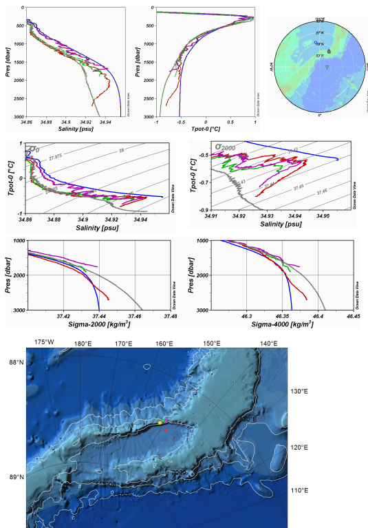
Fig. 18. Potential temperature and salinity profiles and TS curves from stations in the Makarov Basin, the Amundsen Basin and the intra-basin in the Lomonosov Ridge (lower map). In the intra-basin the red station in the interior and the green station at the sill, as well as the stations in the Amundsen and Makarov basins, are taken in 2005 by Oden. The magenta and yellow (not shown in the profiles and TS curves) are taken by Oden in 2001. The 2001 stations indicate that water deriving from the Amundsen Basin deep water was present in the deepest layer, located above the sill depth to the Makarov Basin. If this water crossed the sill it could sink down to 2500 m in the Makarov Basin.
