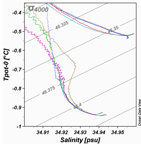
Fig. 17. Deep and bottom water characteristics from the Nansen Basin, Amundsen Basin, Makarov Basin and Canada Basin. Note the absence of a deep temperature minimum in the Makarov Basin and that the temperature minimum observed in the Canada Basin could derive from the Makarov Basin and the deep salinity maximum in the Amundsen Basin could be caused by Makarov Basin deep water crossing the Lomonosov Ridge.
