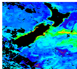
Fig. 11. A case study of phytoplankton bloom detection by PhytoDOAS: the upper panel is a true-color image of MODIS sensor (reported by NASA on 23 December 2009) showing a coccolithophore bloom near Chatham island, on the eastern side of New Zealand. The middle panel depicts the PhytoDOAS retrieval of the coccolithophore chl- a for the same region over a period of two weeks (centered at 23 December 2009). The lower panel illustrates the distribution of MODIS-Aqua PIC for the bloom region as a 8-date composite (19 to 26 December 2009).
