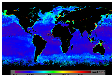
Fig. 8. Comparison of the PhytoDOAS retrieved coccolithophore chl- a [ \text{mg m}^{-3} ] (upper panel) with the NOBM modeled coccolithophore chl- a (middle panel), and the global distribution of MODIS-Aqua PIC [ \text{mol CaCO}_3 \text{m}^{-3} ] (lower panel), all in the northern spring (April/May/June) 2005.
