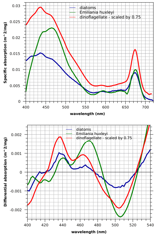
Fig. 2. Upper panel: specific absorption spectra of E. huxleyi (green), dinoflagellates (red) and diatoms (blue). The first two spectra were obtained from cultures using a point-source integrating-cavity absorption meter. The latter spectrum was taken from Bracher et al. (2009). Lower panel: differential absorption spectra of three phytoplankton targets. Each of them was derived by subtracting a second order polynomial from the corresponding specific absorption spectrum, which was shown in upper panel.
