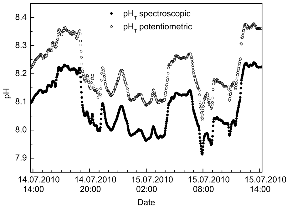
Fig. 8. Comparison of the optically and potentiometrically measured pH for a selected period of 24 h with intense pH variations. Both datasets are converted to the total pH scale at in-situ temperature. The average offset is 0.13 pH units. The last calibration of the glass electrode up to that point was more than a week earlier.
