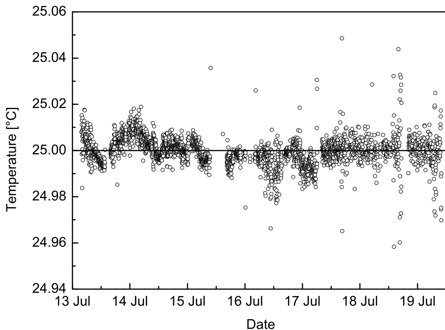
Fig. 3. Tightly controlled sample temperature at 25\text{ °C} \pm 0.006\text{ °C} detected in the cuvette which is a main criterion for precise pH measurements. Temperature regulation is realized by Peltier elements in a preceding heat exchanger (see Fig. 1). Data are from a six-day period during HE331 cruise in July 2010 on R/V Heincke .
