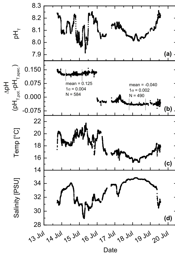
Fig. 9. In-situ data of a cruise in the North Sea from 13 July to 19 July 2010. (a) Optically measured \text{pH}_T . (b) Differences of potentiometric and spectrophotometric measured pH. A calibration of the glass electrode took place at 16 July. Before and after the calibration point, there are two sectors marked for which the mean and standard deviation is calculated. (c) Temperature measured in the FerryBox. (d) Salinity measured in the FerryBox.
