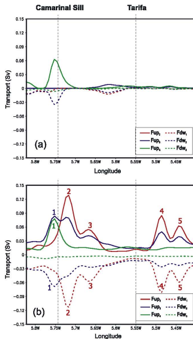
Figure 17. Along-strait time-averaged (on a fortnight period) entrained and detrained volume fluxes between layers (the same as Figure 16) for the case (a) without and (b) with tidal forcing. Positive values (solid lines) indicate upward volume flux, while negative value (dashed lines) represent downward volume fluxes. Positive red, blue, and green lines represent entrainment from L2 to L1, from L3 to L2, and from L4 to L3, respectively. Negative red, blue, and green lines represent entrainment from L1 to L2, from L2 to L3, and from L3 to L4, respectively.
