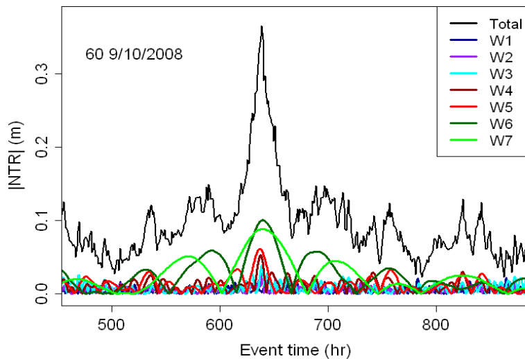
Fig. 1. Magnitude of the NTR wavelet coefficients \Phi_j for an event at Key West on 10 September 2008.
