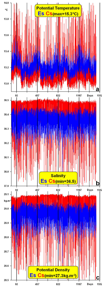
Fig. 2. Original time series of potential temperature (a) , salinity (b) and potential density (c) at Cs (red) and Es (blue) over specified ranges.
