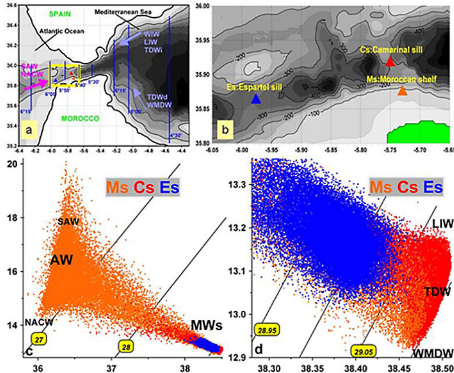
Fig. 1. (a, b) Locations of the CTDs moored at Camarinal Sill (Cs, red triangle, 270 m), on the Moroccan shelf (Ms, orange triangle, 80 m) and at Espartel Sill (Es, blue triangle, 360 m). The blue lines schematise the GIBEX sections (M09) and the waters acronyms are defined in the text. (c) \Theta - S diagrams for the whole 2004–2008 period and over the whole data range of Ms, Cs and Es. (d) \Theta - S diagrams for the whole period and in the MWs ranges at Ms, Cs and Es; WIW is not mentioned since it is roughly located near the AW-TDW mixing line, and is expected to outflow more to the north (M09).
