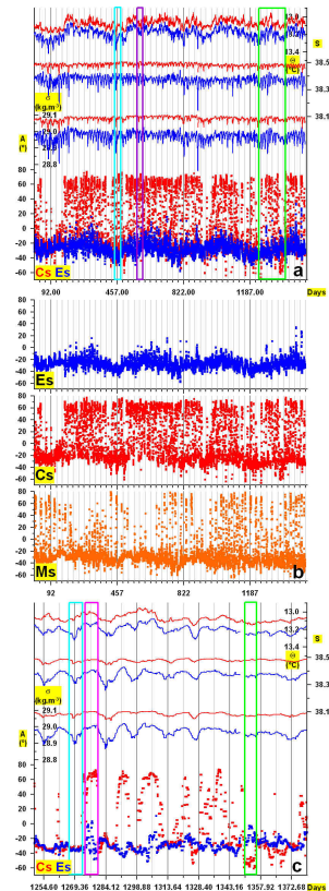
Fig. 3. (a) Time series (25-h median values) at both Cs (red) and Es (blue) during the whole period (d1–d1490); on the time axis, major grid lines (dark grey on d92, ...) are on January 1st and minor grid lines (light grey) are one month apart. Coloured periods correspond to data plotted in Fig. 4b (cyan), Fig. 4c (magenta) and Fig. 3c (green). Ticks on the vertical axes indicate the overall ranges for the measured parameters \Theta (descending axis), S and \sigma as well as the range of interest for the computed slope A of the temporal mixing lines. (b) Computed slope A of the temporal mixing lines at Es, Cs and Ms. (c) A s for (a) during the period specified in green in (a) (d1250–d1380); on the time axis, major grid lines (dark grey) indicate spring tide, minor grid lines (light grey) indicate neap tide, both being plotted 14.76 days apart. Coloured periods correspond to data plotted in Fig. 4d (cyan), Fig. 4e (magenta) and Fig. 4f (green).
