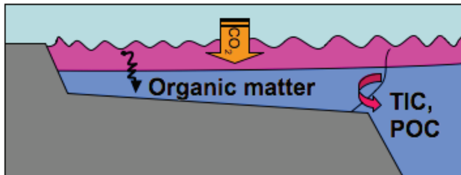
Fig. 3. The biological Continental Shelf Pump mechanism.
