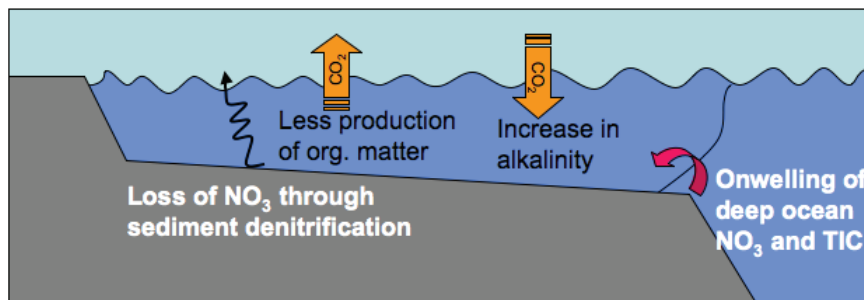
Fig. 8. The two opposing effects of sediment denitrification on the biological CSP. On the one hand, removal of fixed nitrogen reduces the production of organic matter, which should correspond to a net efflux of \text{CO}_2 . On the other hand, denitrification generates alkalinity and lowers p\text{CO}_2 , which should lead to uptake of atmospheric \text{CO}_2 .
