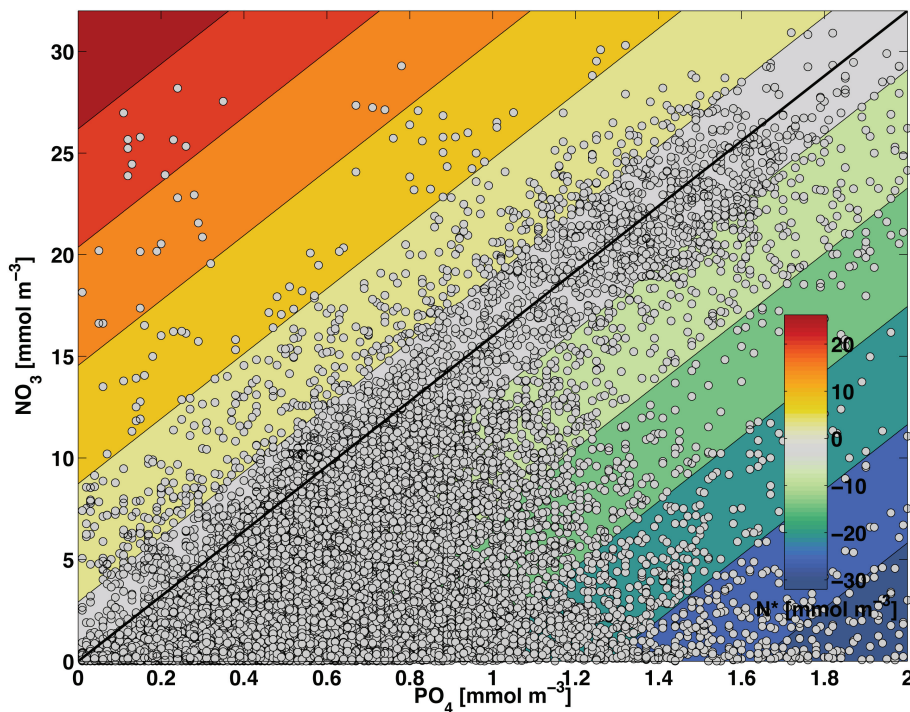
Fig. 5. Nitrate plotted over phosphate for 25 790 samples from the MAB shelf. Samples were taken during cruises undertaken by Brookhaven National Laboratories and during the SEEP and OMP programs (see text for details). \text{N}^* , given in color, quantifies the nitrogen excess/deficit with respect to phosphate. The bold line marks \text{N}^*=0 and corresponds to the Redfield ratio of 16:1.
