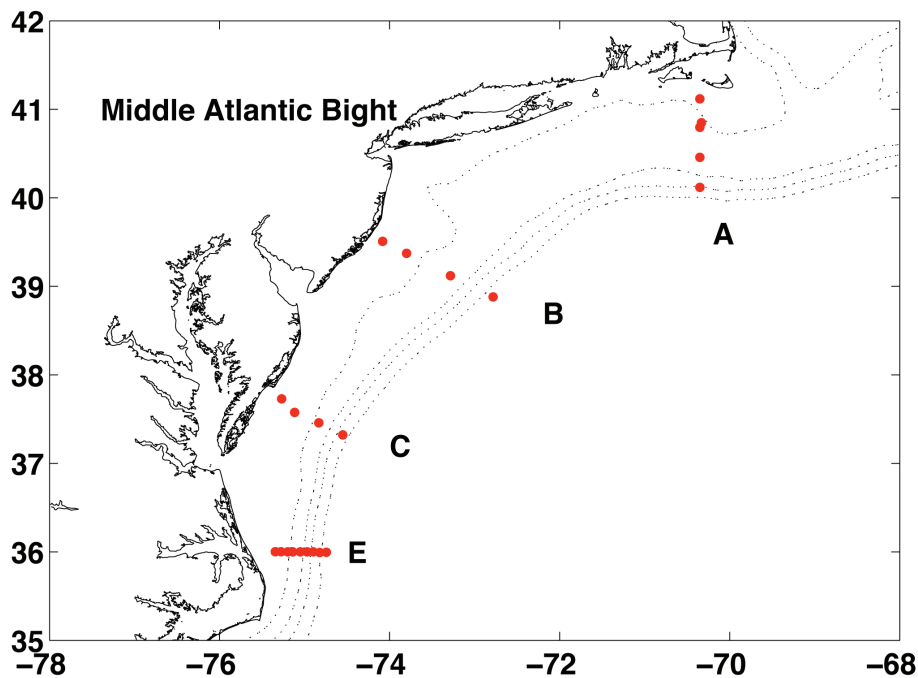
Fig. 6. Location of stations on four transects that were sampled during the OMP program. N^* along these transects are shown in Fig. 7.
