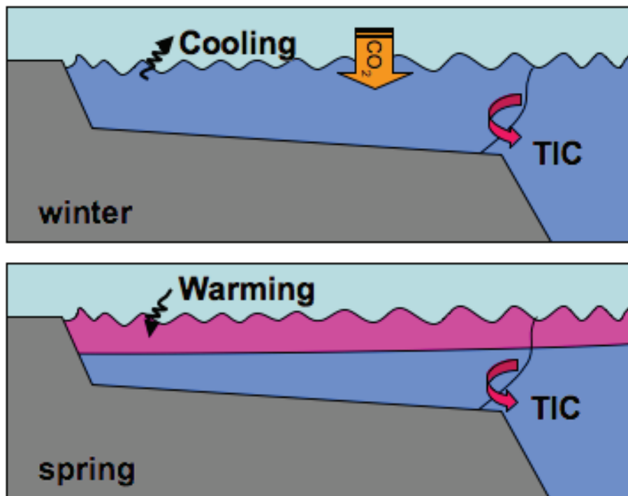
Fig. 2. The physical Continental Shelf Pump mechanism.
