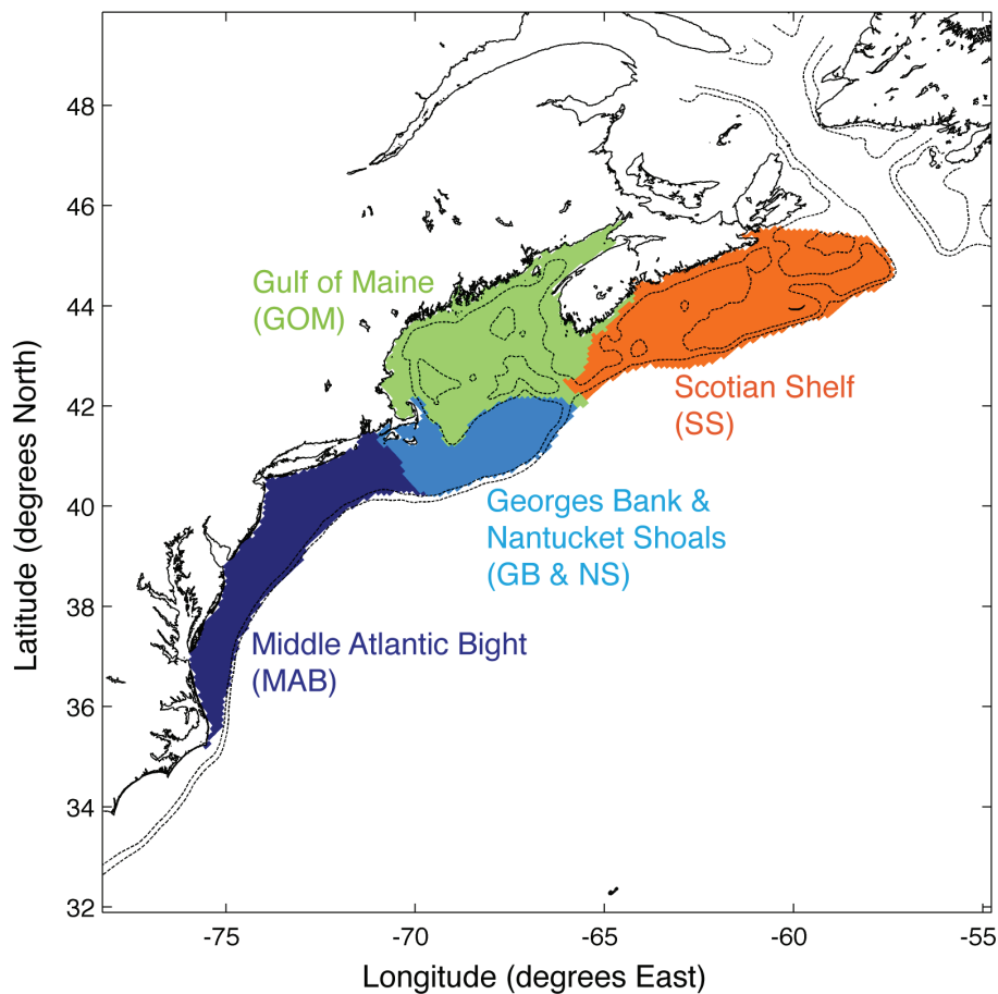
Fig. 4. Geographic shelf regions used for budgets. The dashed lines show the 100 m and 200 m isobaths.
