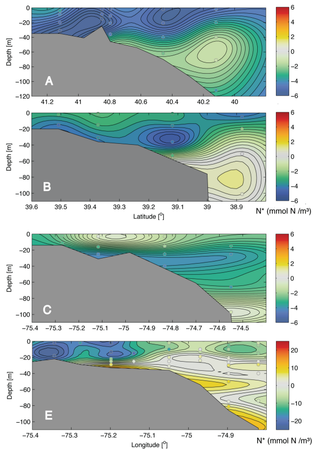
Fig. 7. N^* along four transects on the MAB shelf (see Fig. 6 for station locations). The contour plots show optimally interpolated fields. The location of data points is shown by the colored circles; the color within circles indicates the observed value.
