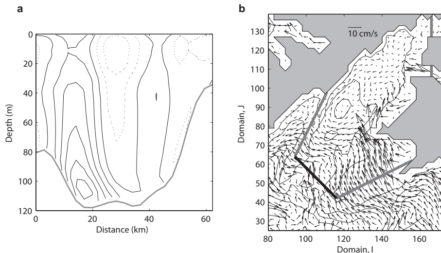
Fig. 7. (a) Difference from mean cross-sill velocity for cases of strong outflow (cross-sill velocity u_{\text{out}} > 20 \text{ cm s}^{-1} ). Contour lines are drawn in 2.5 \text{ cm s}^{-1} increments. Solid lines denote flow directed out of the fjord and zero flow, dotted lines denote flow into the fjord. (b) Difference from mean surface circulation in Storjorden for cases of strong outflow. Isobaths are drawn at 50 m intervals. Thick lines delineate the Storjorden basin. The thick black line marks the position of the sill.
