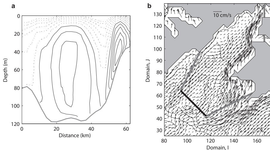
Fig. 9. (a) Difference from mean cross-sill velocity for times of east-southeasterly winds (90–135 °T, 64 of 365 days). Contour lines are drawn in 1 \text{ cm s}^{-1} increments. Solid lines denote flow directed out of the fjord and zero flow, dotted lines denote flow into the fjord. (b) Difference from mean surface circulation in Storfjorden for times of southeasterly to easterly winds. Isobaths are drawn at 50 m intervals. Thick lines delineate the Storfjorden basin. The thick black line marks the position of the sill.
