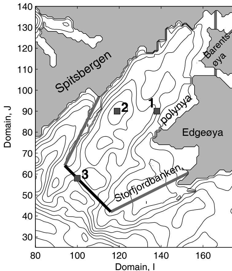
Fig. 2. Storfjorden with stations 1–3 (squares), thick lines delimit the extent of the Storfjorden basin. The black thick line is the Storfjorden sill. Station 3 is positioned at the site where the main overflow occurs across the sill. Isobaths are drawn at 25 m intervals. The center of the polynya area close to Edgeøya is indicated.
