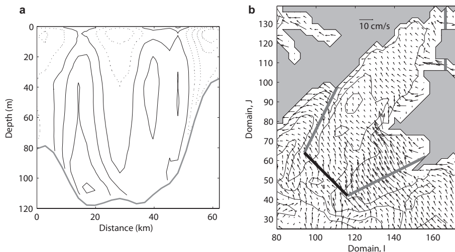
Fig. 8. (a) Difference from mean cross-sill velocity for times of east-northeasterly winds (45–90°T, 86 of 365 days). Contour lines are drawn in 1 \text{ cm s}^{-1} increments. Solid lines denote flow directed out of the fjord and zero flow, dotted lines denote flow into the fjord. (b) Difference from mean surface circulation in Storfjorden for times of easterly to northeasterly winds. Isobaths are drawn at 50 m intervals. Thick lines delineate the Storfjorden basin. The thick black line marks the position of the sill.
