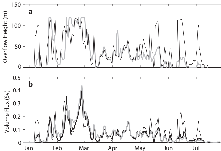
Fig. 13. (a) Comparison of overflow height calculated from velocity profiles following the method detailed in Geyer et al. (2009) (black) with overflow height directly determined by velocity profiles and water mass properties (grey). (b) Comparison of overflow volume flux estimates from determined using overflow height estimate and constant overflow width of 15 km (thin black line) and correct overflow height and constant overflow width of 15 km (thick black line), respectively, with directly determined overflow volume transport (grey).
