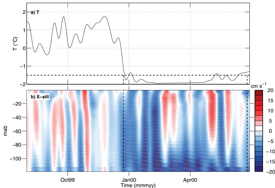
Fig. 3. Time series of (a) bottom temperature and (b) cross-sill component of the velocity (negative values out of the fjord) at station 3. 15-day low-passed data are shown. Vertical dashed lines mark the start and end of the overflow season.
