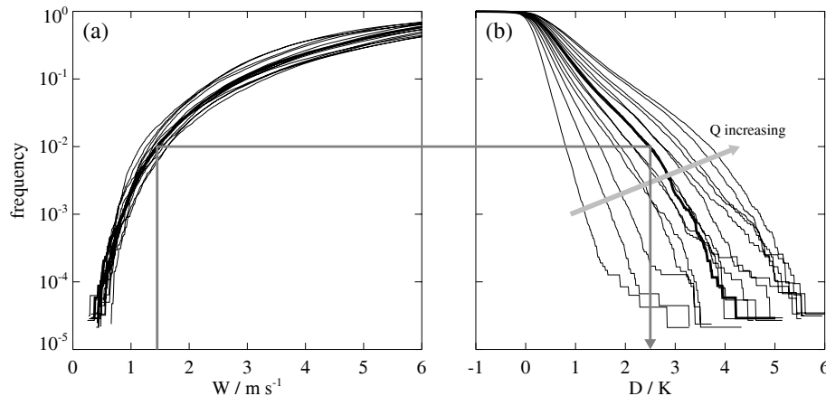
Fig. 1. Example of direct frequency matching, for 14:00 LT. (a) Maximum in wind speed ( W ) distribution. (b) Warming ( D ) distribution. Each curve corresponds to a different integrated heat flux ( Q ) bin; Q ranges from 4.2 to 17 \text{ MJ m}^{-2} . For a given frequency, curves for larger Q tend to give larger D . Note that there is covariance of W and Q (from varying atmospheric stability and varying sensible and latent heat fluxes) and this is included in the resulting model. The concept of frequency matching is that (following the thin grey arrow), for a particular Q bin (bold curves), persistent wind speeds less than 1.4 \text{ m s}^{-1} occur with frequency 10^{-2} in the NWP data, which corresponds to the frequency of warming greater than 2.5 K.
