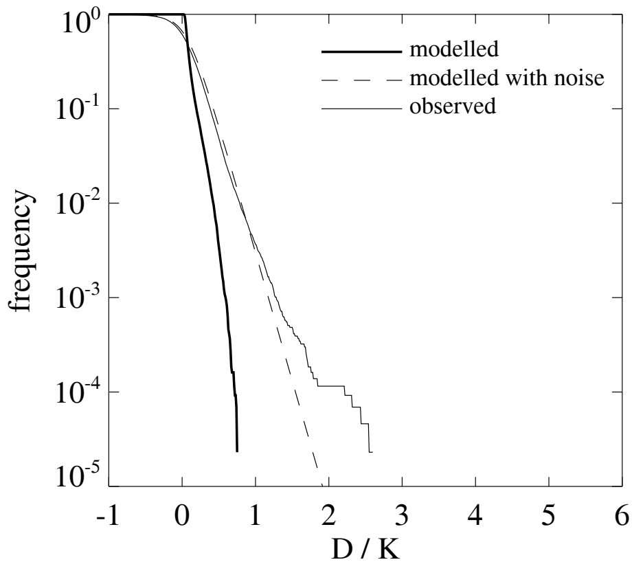
Fig. 4. Fit between the probability distributions of modelled warming and observed warming D at 18:00 LT for small integrated heat flux ( 4.3 \text{ MJ m}^{-2} ). The modelled warming ranges from zero to 0.8 \text{ K} . When the background noise is added, the modelled distribution matches the observed distribution. The fit is poor at the very largest values of warming but does include non-zero probability of negative D .
