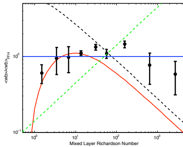
Figure 1: Simulation data for \overline{w'b'} , rescaled by the FFH expectation. The lines indicate expectations of different theories: blue solid for FFH, red solid for CD, green dashed for Green (1970), and black dashed for Stone (1972b).
