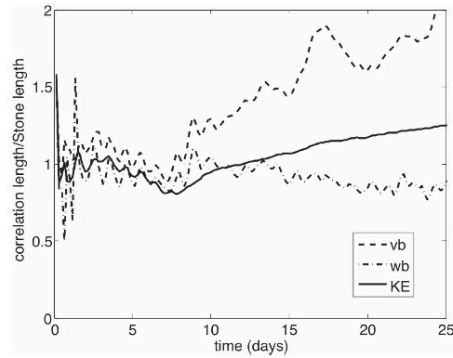
FIG. 9. The horizontal length scales typical of the correlations v'b' , w'b' , and EKE for the same simulation as in Fig. 4, are compared to the most unstable length scale. Length scales from the v' and b' cospectrum, the w' and b' cospectrum, and the EKE spectrum, E(k) , are shown rescaled by the time-evolving L_s ; L_s^2 = \int \Re[S(k)] dk / \int k^2 \Re[S(k)] dk for a cospectrum S(k) , and the \int \Re[S(k)] dk is the full correlation. For more details on cospectra, see Emery and Thomson (2001).
