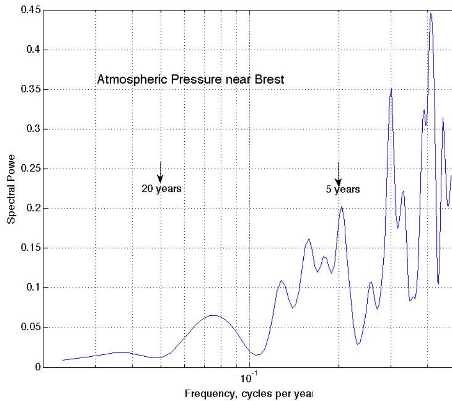
Fig. 1. Spectrum of Atm Pressure at Brest
