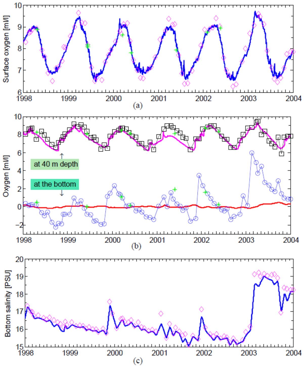
Figure 6. Time series at BY5 for the period 1998-2003. Calculated results are presented with a thick solid line and observation data of BED and FIMR with symbols (see capture of Fig. 5 for more details). (a) – surface oxygen; (b) – oxygen at 40 m depth and at the bottom; (c) - bottom salinity.
