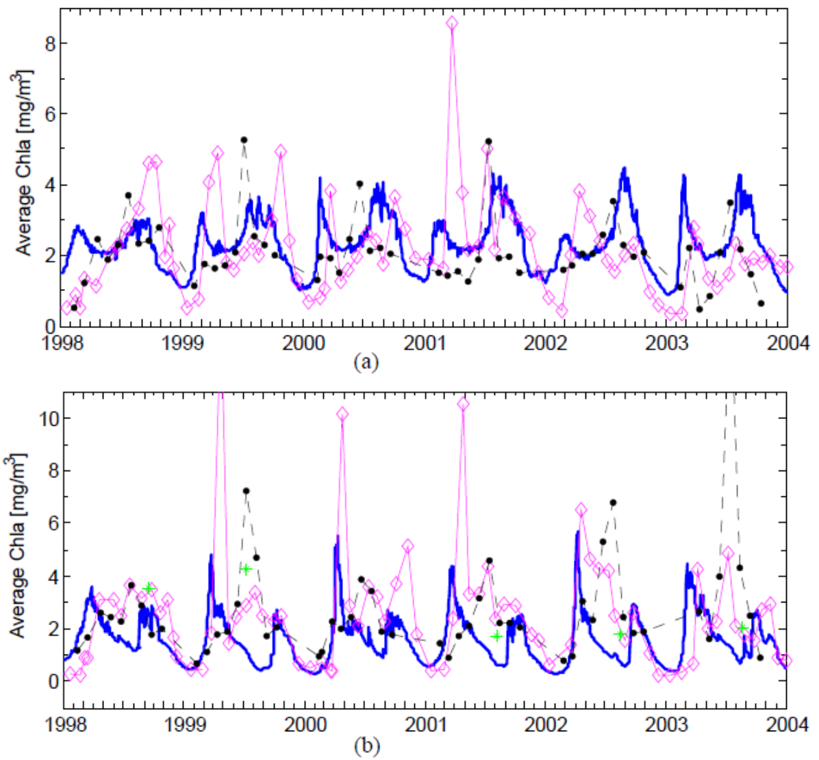
Figure 9. Modelled (thick solid line) and in-situ data (denoted with blank diamonds and asterisks) of average Chla [mg/m 3 ] at: (a) - BY5, (b) - BY15. Data from satellite images (EMIS database) is presented with filled circles connected with a dash line.
