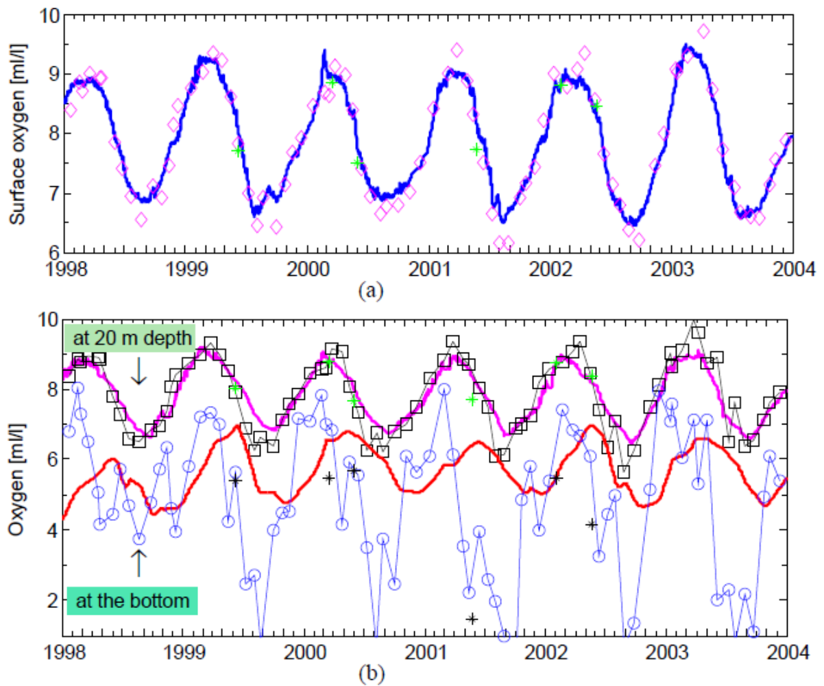
Figure 7. Oxygen time series at BY1 for the period 1998-2003. Calculated results are presented with a thick solid line and observation data of BED and FIMR with symbols (see capture of Fig. 5 for more details). (a) – surface oxygen; (b) – oxygen at 20 m depth and at the bottom.
