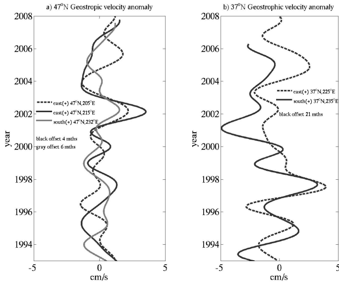
Fig. 13. Geostrophic velocity anomalies at 2 latitudes: a) zonal velocity at 47°N, 205°E (black dashed line), 47°N and 215°E (black solid line) offset by 4 months, and meridional velocity at 47°N, 232°E, offset by 6 months; b) zonal velocity at 37°N, 225°E (black dashed line) and meridional velocity at 37°N, 235°E, offset by 21 months. Annual and higher frequencies have been removed. Offsets determined by lag of maximum correlation in time series between the time series.
