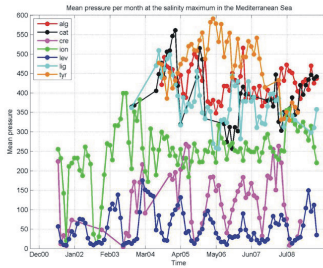
Fig. 2. Depth of salinity maximum in the Mediterranean basin between December 2000 and June 2009 computed from float data (Notarstefano and Poulain, 2009).
