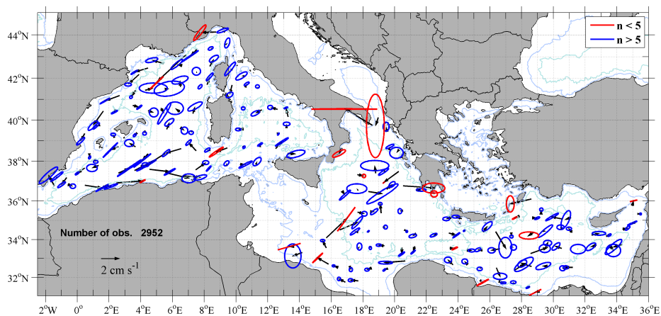
Fig. 1. Mean intermediate currents and standard error ellipses computed from float data.
