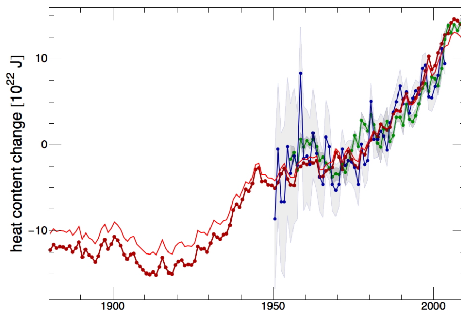
Fig. 3. Fig. 3. Heat content change calculated using the Munk value Az \approx 1.3 \times 10^{-4} \text{ m}^2/\text{s} for eddy diffusivity (thick red) and using Az \approx 0.9 \times 10^{-4} \text{ m}^2/\text{s} (thin red). Blue: Domingues et al., Green: Levitus et al.
