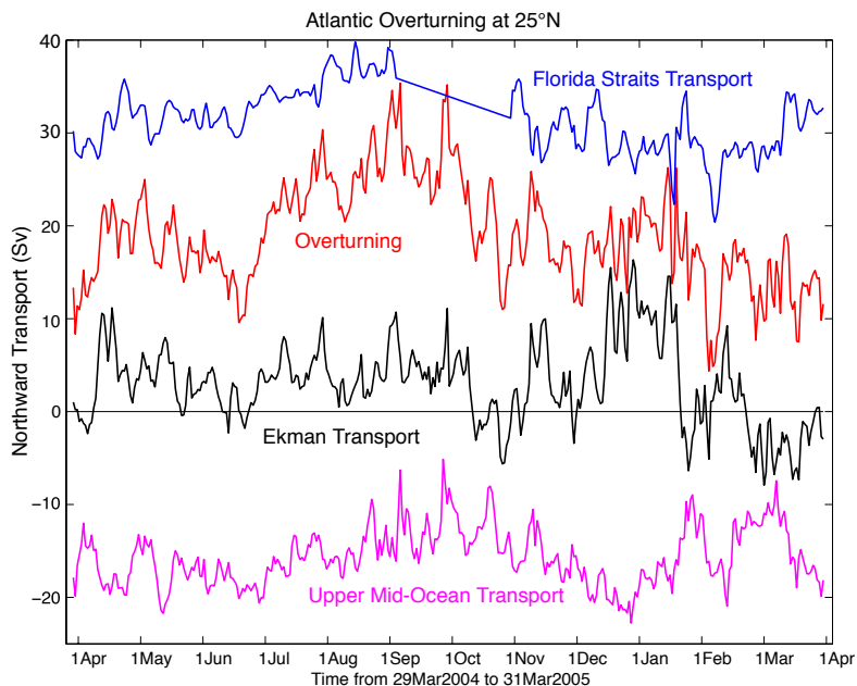
Fig. 2. Daily time series of Florida Straits transport (blue), Ekman transport (black), upper mid-ocean geostrophic transport (magenta) and overturning transport (red) for the period 29 March 2004 to 31 March 2005. Florida Straits transport is based on electromagnetic cable measurements. Ekman transport is based on QuikScat-determined winds. The geostrophic transport is based on Rapid times series of dynamic height at the eastern and western boundaries of the 25° N section and the reference level velocity is set by forcing the geostrophic transport to equal the Florida straits plus Ekman transport on a daily basis. Upper mid-ocean transport is the vertical integral of the transport per unit depth down to the deepest northward velocity (approximately 1100 m depth) on each day. Overturning transport is then the sum of the Florida Straits, Ekman and upper mid-ocean geostrophic transports and represents the maximum northward transport of upper layer waters on each day.
