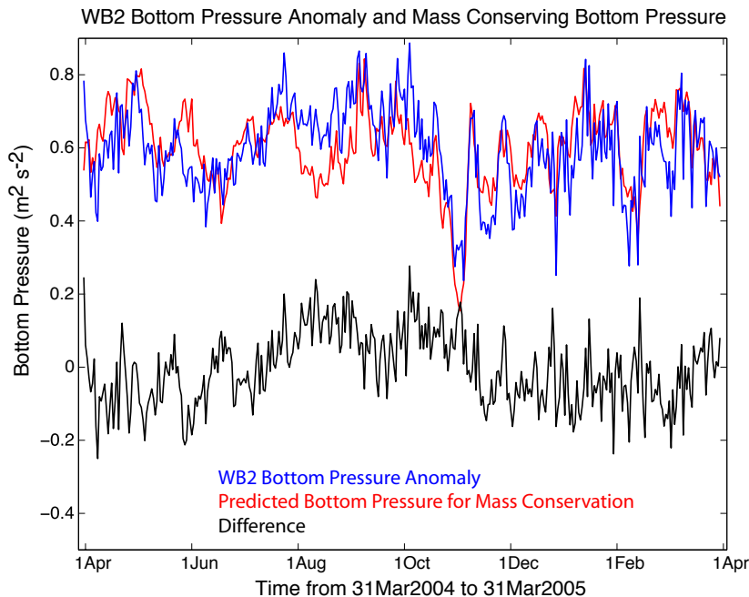
Fig. 7. Bottom pressure at wb2. The bottom pressure anomaly (blue) is defined to be the bottom pressure measured at wb2 minus the zonal average bottom pressure shown in Fig. 4. Predicted bottom pressure (red) is that required to compensate for local baroclinic transport variability shown in Fig. 5. The difference between bottom pressure anomaly and predicted bottom pressure at wb2 is shown in black. The blue and red curves have been offset from the black curve by adding 0.06 dbar to them.
