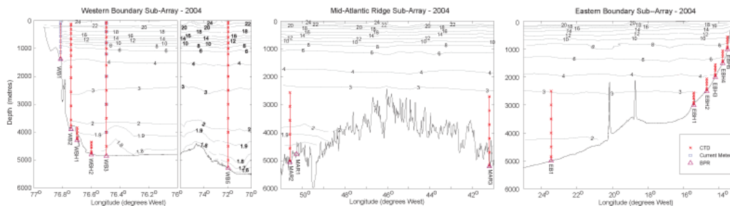
Fig. 3. Rapid Array along 26.5^{\circ} N during 2004–2005. Only instruments that returned year-long time series are shown. Principal components are 15 bottom pressure records and 12 dynamic height moorings concentrated near the western and eastern boundaries.
