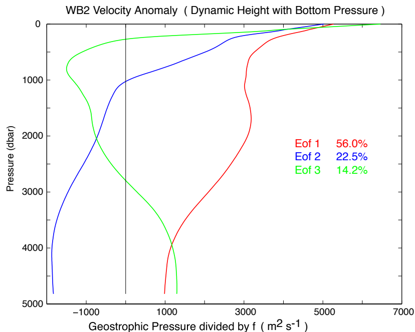
Fig. 10. Empirical orthogonal functions for the vertical structure in geostrophic pressure divided by f at wb2. Bottom pressure anomaly (difference between measured bottom pressure and zonally averaged bottom pressure) is added to the dynamic height anomaly profile at each day to estimate geostrophic pressure which is then divided by the Coriolis parameter to generate a profile of transport per unit depth in \text{m}^2 \text{s}^{-2} . The first 3 eof's illustrate the vertical structure in the daily time series.
