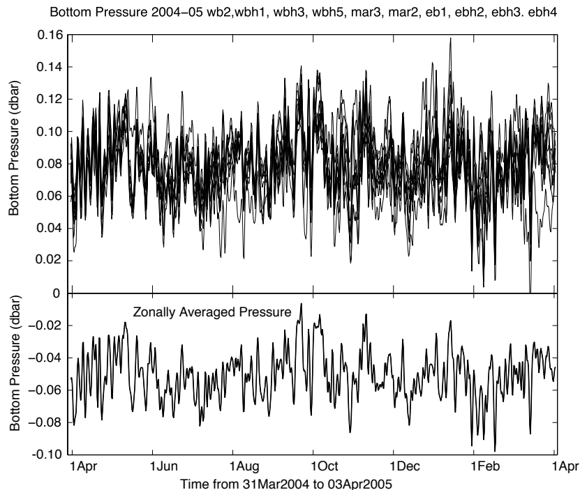
Fig. 6. Bottom pressure time series: (a) at 10 sites across the Atlantic at 26.5^{\circ} N (each offset by 0.08 dbar) and (b) the zonal average bottom pressure on each day (offset by -0.05 dbar). Note that bottom pressure appears to rise and fall in phase at all 10 sites.
