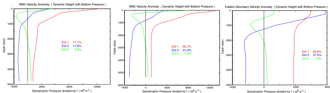
Fig. 11. Empirical orthogonal functions for the vertical structure in geostrophic pressure divided by f at moorings wb3 (a), wb5 (b) and ebh (c).
