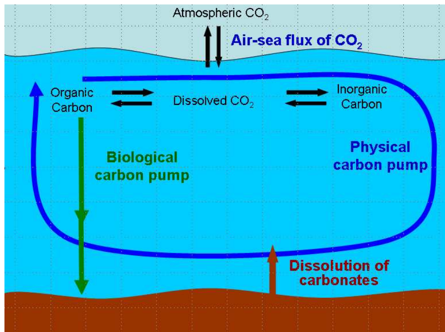
Fig. 1. Schematic of the oceanic carbon cycle, including air-sea flux, biological pump, physical pump and dissolution of carbonates.
