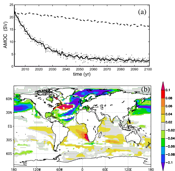
Fig. 2. (a) Maximum AMOC at 35°N (Sv) of all hosing ensemble members, together with their ensemble mean (solid). The standard ensemble mean (dashed) is given for comparison. (b) Regression of the difference in SST between the hosing and standard runs on the difference in maximum AMOC at 35°N (°C/Sv) for 2000–2050. A 5-yr running mean has been applied to the data before regressing. Shading as in Fig. 1.
