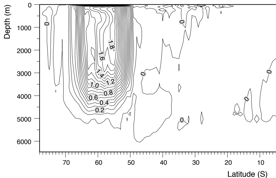
Fig. 4. Difference in the meridional overturning streamfunction between the perturbation run (Run 2 – an additional 0.1 \text{ dyne cm}^{-2} wind stress at the latitudes of Drake Passage) and the control run after two days.
