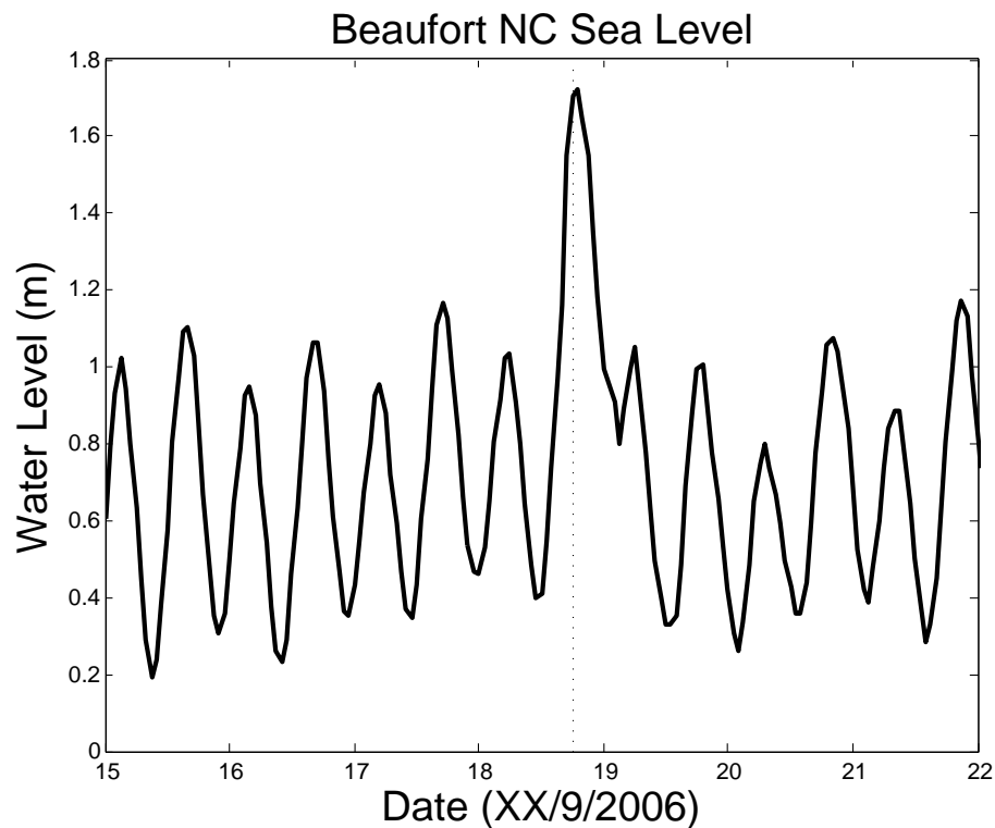
Fig. 6. Sea level at Beaufort Inlet, NC.
