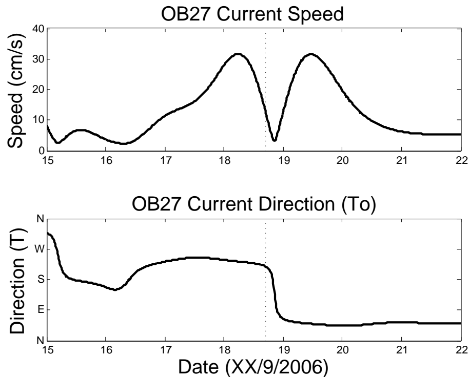
Fig. 9. Low pass current speed and direction at OB27. Small dotted lines show time of landfall.
