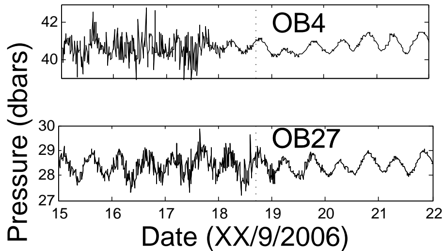
Fig. 5. Bottom pressure at OB4 and OB27. Small dotted lines show time of landfall.
