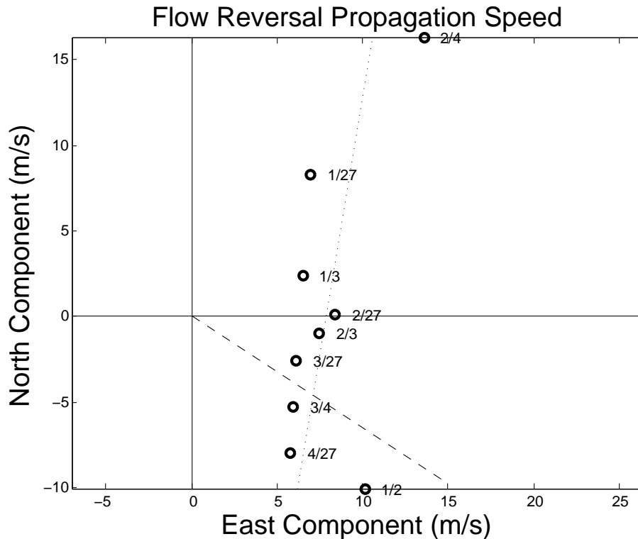
Fig. 10. Propagation of the flow reversal across the CORMP array. Individual points are labeled with the appropriate pair of moorings. For example, point labeled “1/27” shows the speed and direction of propagation of the flow reversal from OB1 to OB27. Dotted line is a least squares fit to the points shown. Dashed line points 33° below the x-axis, approximately the offshore direction.
