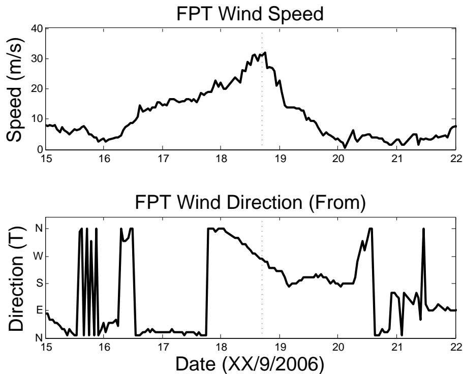
Fig. 7. Wind speed and direction at FPT. Small dotted lines show time of landfall.
