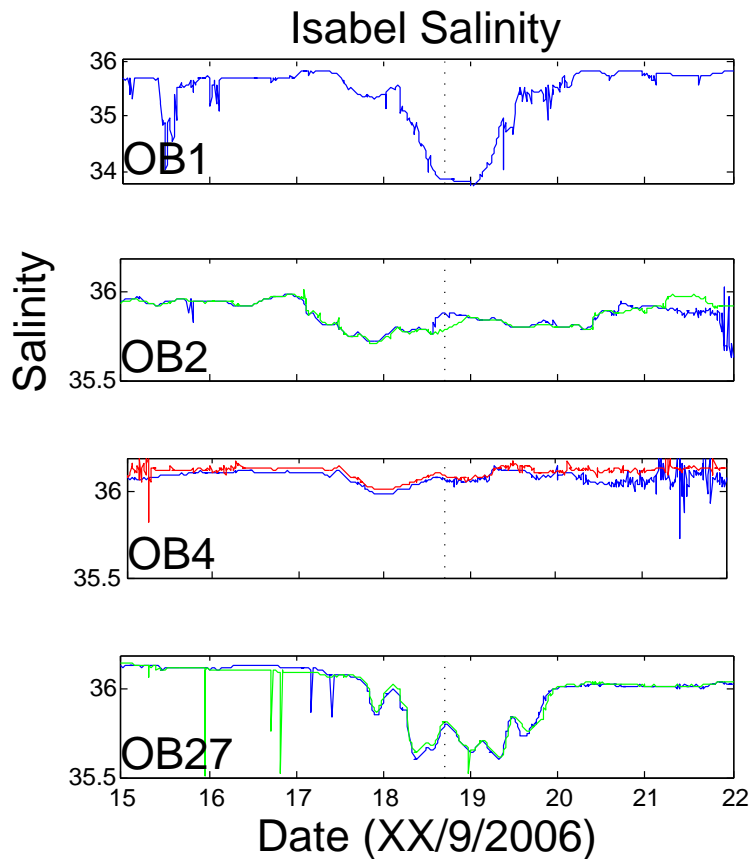
Fig. 4. As in Fig. 2, but for salinity. Note some records are not plotted because data were not of acceptable quality to present (see Table 1). Small dotted lines show time of landfall.
