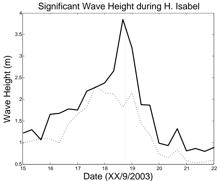
Fig. 12. Significant wave height (m) at OB1 (solid) and OB3 (dashed). Small dotted lines show time of landfall.
