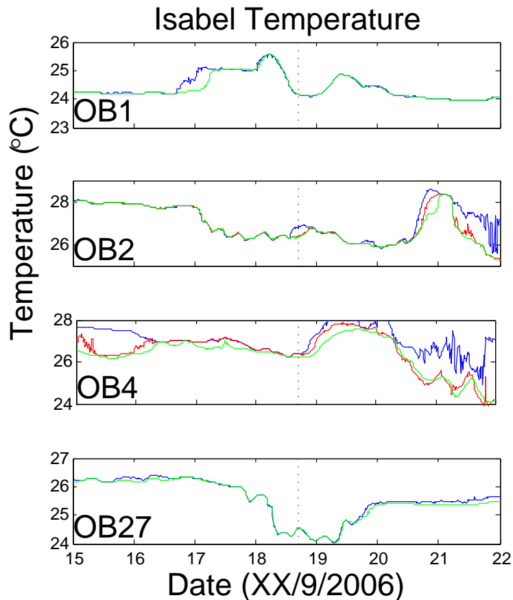
Fig. 2. Temperature at 4 moorings during the period surrounding the landfall of Hurricane Isabel. Green curves are lower or bottom instruments. Blue curves are upper or 15 m instruments and red curves are lower or 30 m instruments (see Table 1). Note different temperature scales for different moorings. Small dotted lines show time of landfall.
