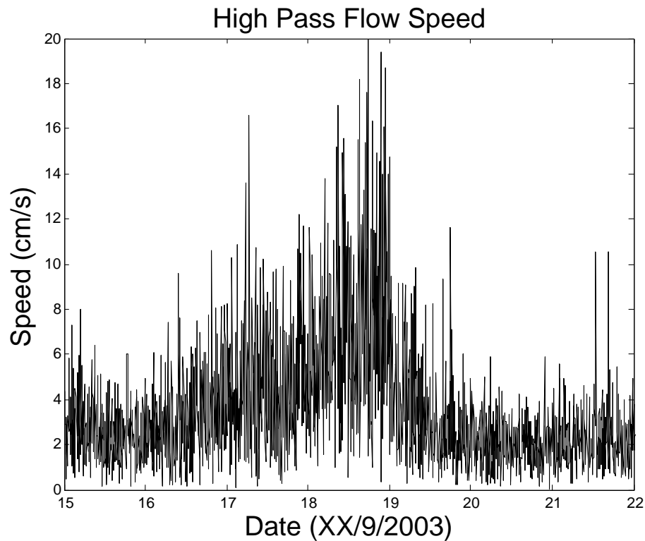
Fig. 11. Speed of the high pass flow at OB27.
