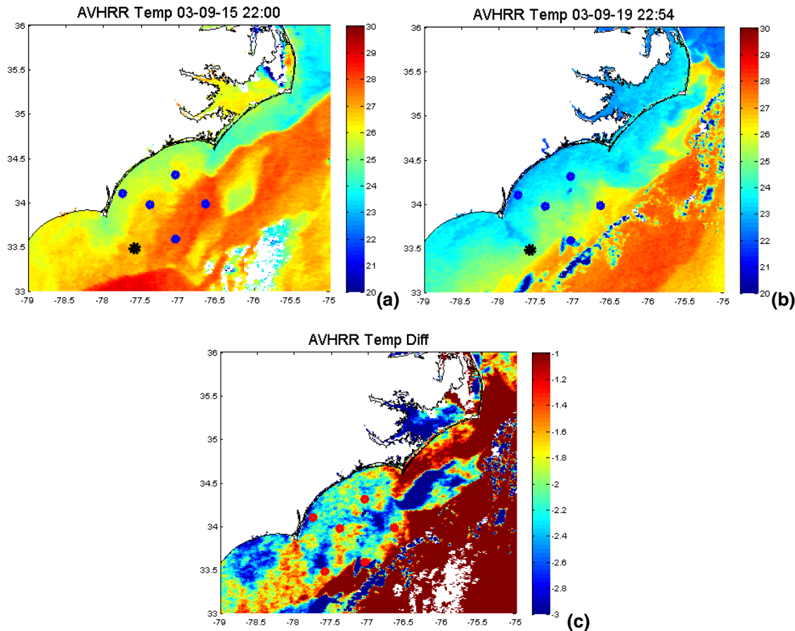
Fig. 3. (a) AVHRR MCSST Temperature ( ^{\circ}\text{C} ) image from 15 September 2003 at 22:00. Color-bar at right indicates temperature scale. Locations of CORMP moorings and FPT are shown on map (see Fig. 1). (b) Same as (a) but for 19 September 2003 at 22:54. (c) Temperature difference between (a) and (b).
