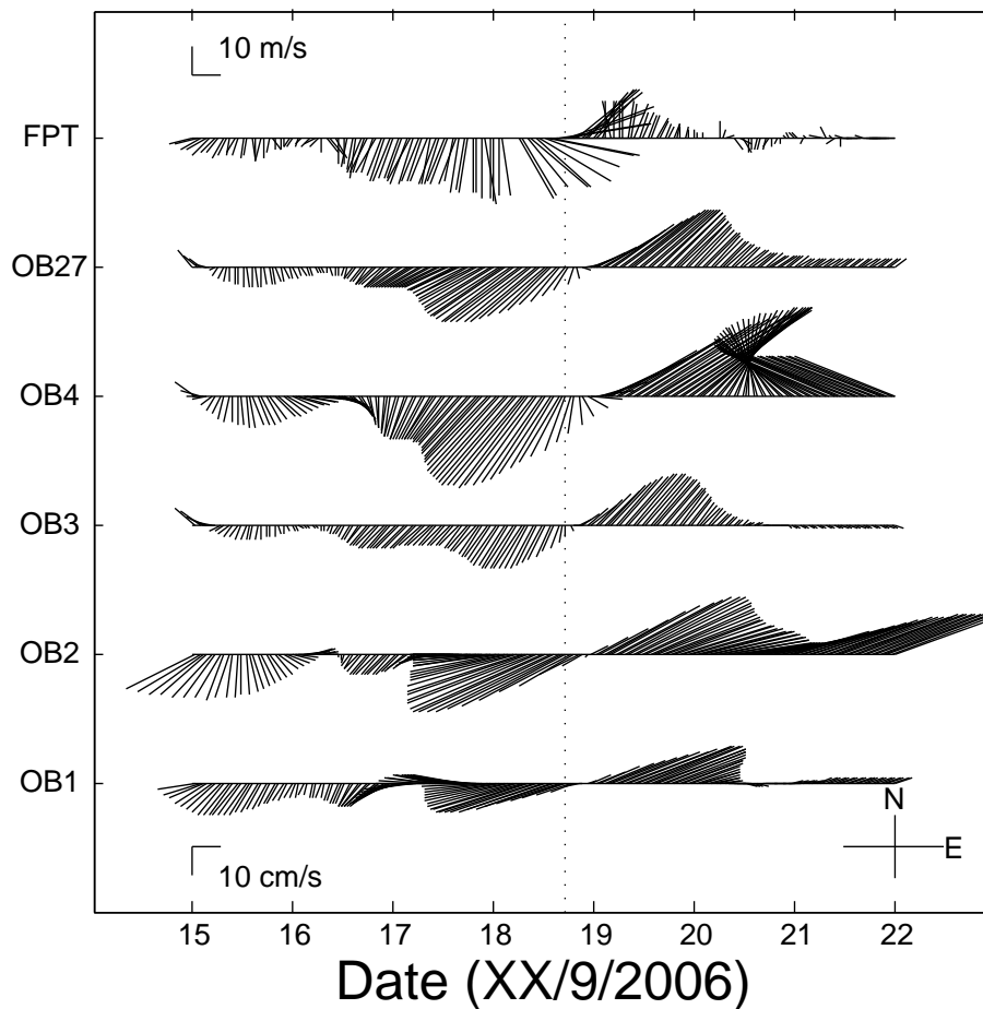
Fig. 8. Stick diagram of winds at FPT (top series) and low-pass currents at other moorings as shown at left. A scale for the winds is shown at the top left and for the currents at bottom left.
