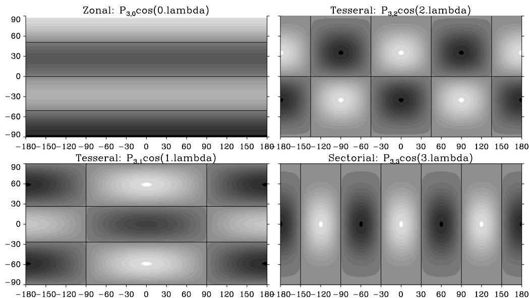
Fig. 1. Four of the seven spherical harmonics of degree 3. The remaining three are produced by shifting the patterns to the east by a quarter of a zonal wavelength. The number of circular nodal lines (horizontal lines plus half the number of vertical lines) is three in each case.
