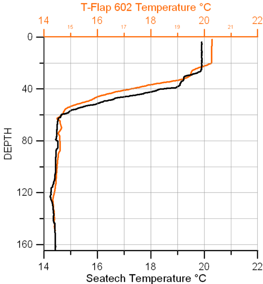
Fig. 11. Comparison between temperature measurement of T-FLAP (orange line) and reference probe (black line ).
