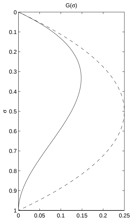
Fig. 7. Vertical profile of the shape function G(\sigma) , where \sigma = -z/h , in the special case G(1) \sim dG/d\sigma|_{\sigma=1} \sim 0 . Solid line is the original cubic, dashed line is the simplified quadratic form.
