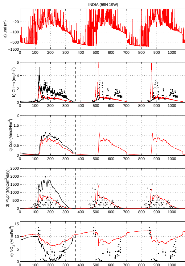
Fig. 4. Annual cycle of modelled (solid line) and observed (dots) ecosystem characteristics at station India: (a) – UML depth (m) (note log-scale), (b) – UML depth integrated Chl-a ( \text{mg Chl m}^{-3} ), (c) – surface zooplankton biomass ( \text{mmol N m}^{-3} ), (d) – UML integrated primary production ( \text{g C m}^{-2} \text{d}^{-1} ), (e) – surface nitrate concentration ( \text{mmol N m}^{-3} ). Results of the numerical experiment are shown for the first year as a thick line.
